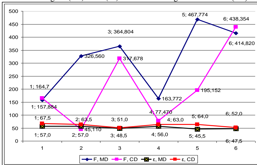
Graph 1: Tensile strength F(md) and F(cd) and tensile elongation at break \varepsilon(md) and \varepsilon(cd)
