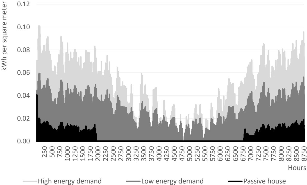
Figure 2: Hourly heating demand time series for one year for three different building archetypes
