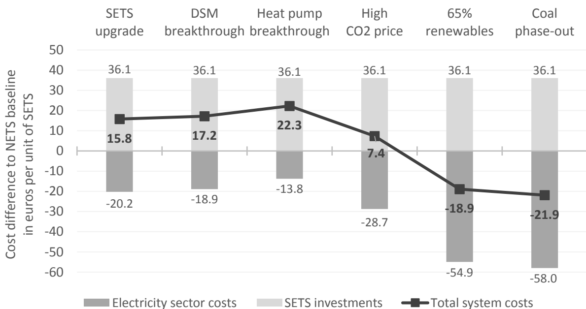
Figure 3: Specific system cost effect per SETS unit from upgrading NETS to SETS in the central scenarios
