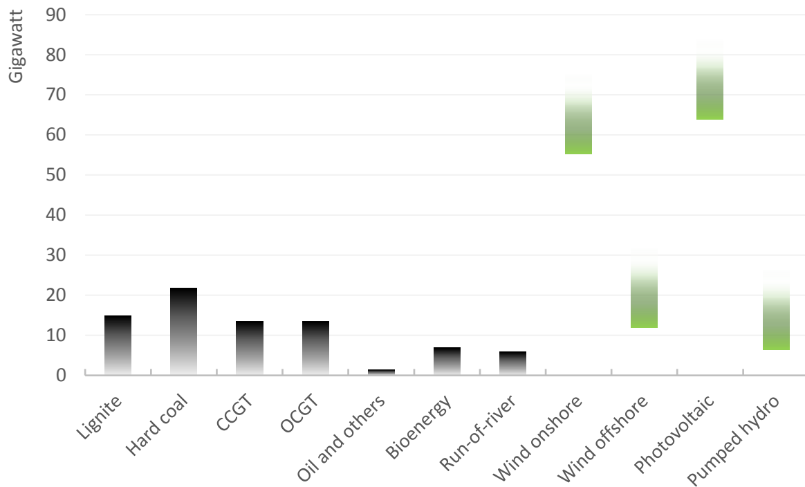
Figure 1: Assumptions on upper and lower bounds for the generation portfolio
