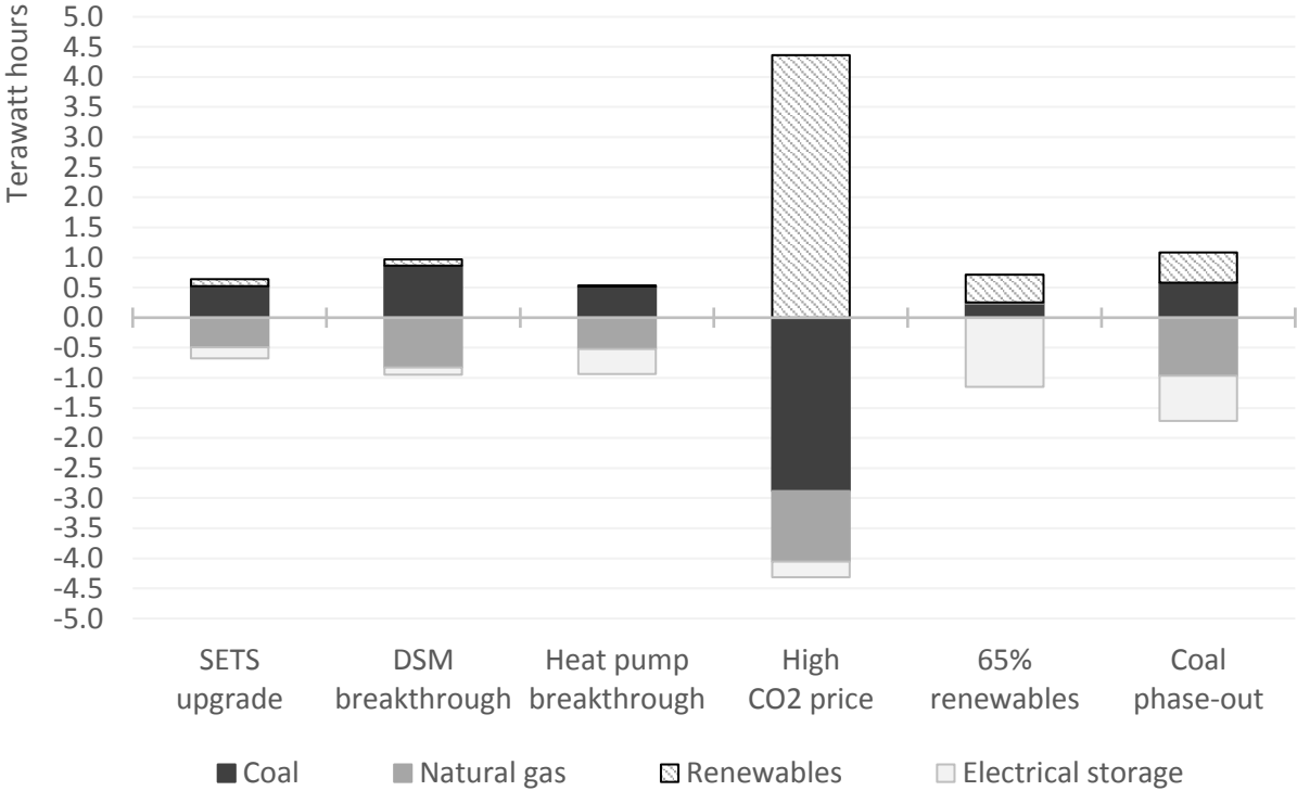
Figure 6: Differences in annual electricity generation compared to the respective NETS baselines
