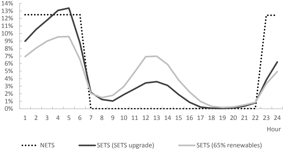
Figure 10: Average daily charging pattern of NETS and SETS
