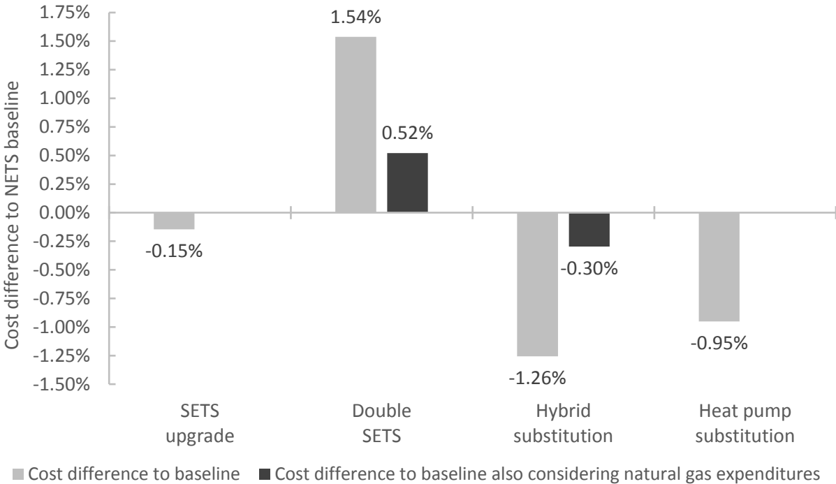
Figure 14: Electricity sector cost effects for further scenarios with alternative assumptions on heating technologies
