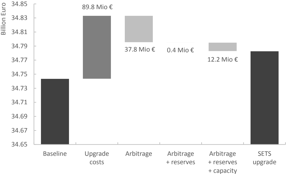
Figure 8: Waterfall separation of SETS system values in the central SETS upgrade scenario
