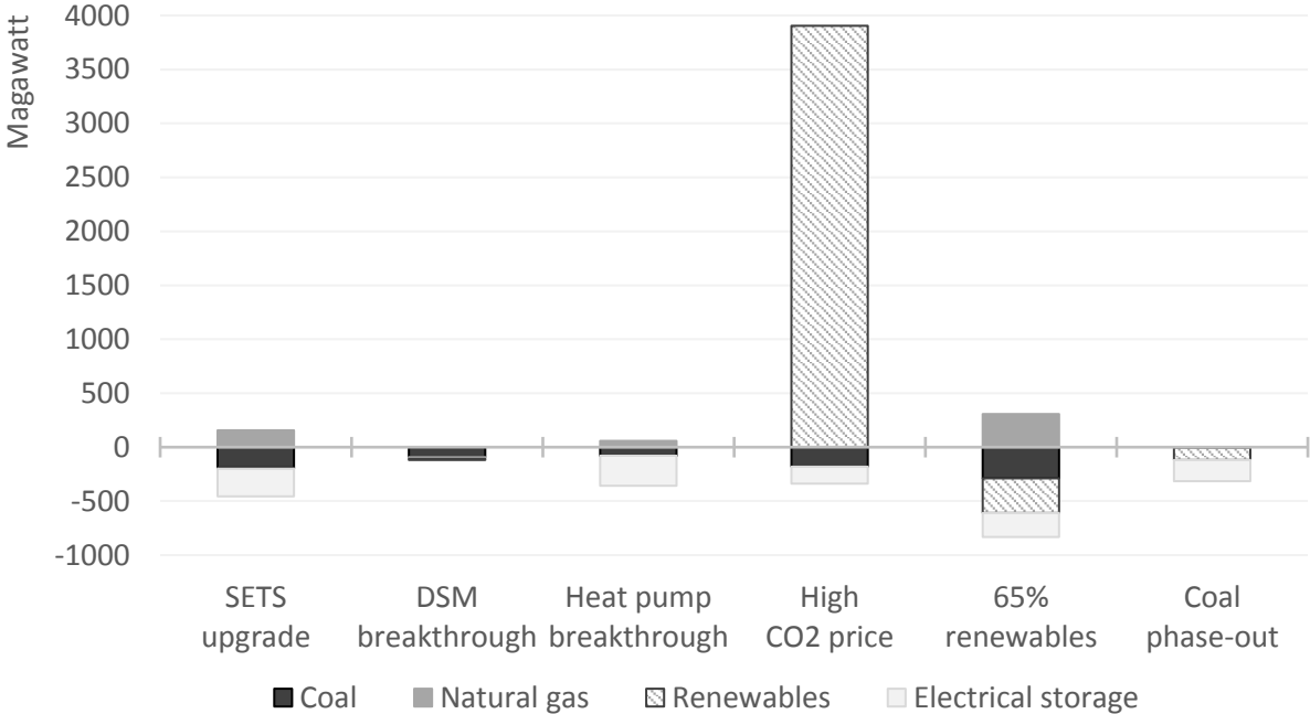
Figure 5: Differences in installed generation and storage capacities compared to the respective NETS baselines
