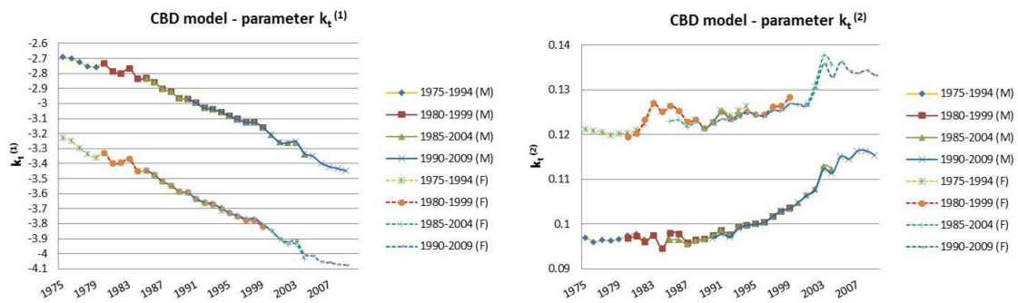
Figure 13. CBD Jumping Fixed-Length-Horizon: parameter estimates.
