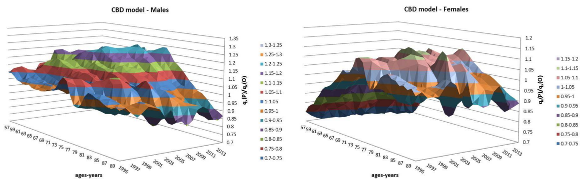
Figure 8. Cairns–Blake–Dowd Fixed Horizon Backtest: \frac{q_{x,t}^P}{q_{x,t}^O} ratio.
