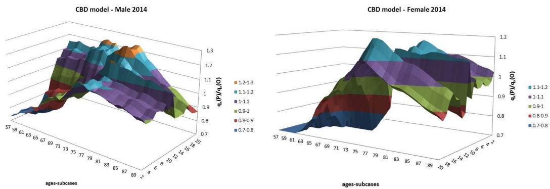
Figure 16. CBD Rolling Fixed-Length Horizon Backtests: \frac{q_{x,t}^P}{q_{x,t}^O} ratio 2014.
