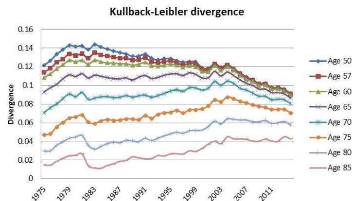
Figure 2. Kullback–Leibler divergence with respect to Z_\zeta at selected ages.
