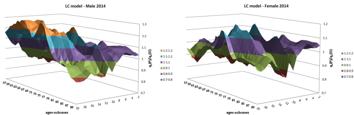
Figure 15. LC Rolling Fixed-Length Horizon Backtests: \frac{q_{x,t}^P}{q_{x,t}^O} ratio 2014.
