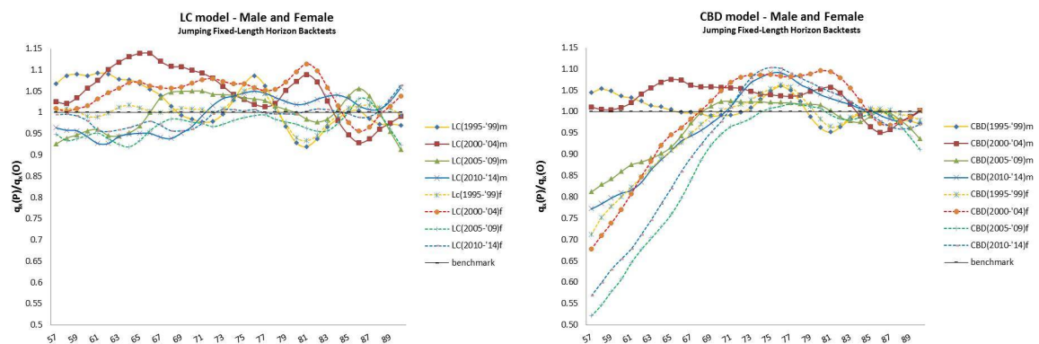
Figure 12. LC and CBD \frac{q_{x,t}^p}{q_{x,t}^O} ratio: comparison between models. Note: the curves represent the average of the \frac{q_{x,t}^p}{q_{x,t}^O} ratio over the five-years forecast horizon.
