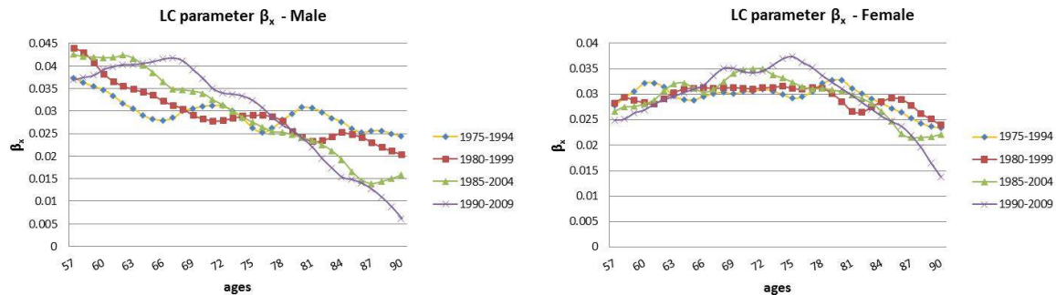
Figure 11. LC Jumping Fixed-Length-Horizon: \beta_x parameter estimates.
