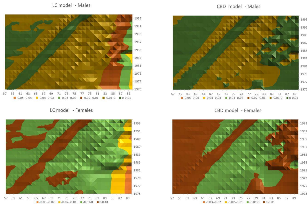
Figure 4. Residuals ( q_{x,t}^O - q_{x,t}^P ) by age x : 1975–1994.
