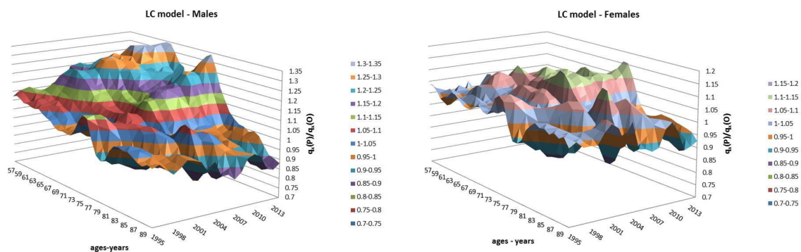
Figure 6. Lee–Carter Fixed Horizon Backtest: \frac{q_{x,t}^P}{q_{x,t}^O} ratio.
