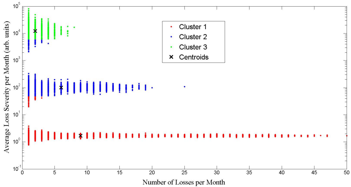
Figure 4. DPFS for Scenario (I); three distinct regions are found between frequency and severity; centroids are marked with an “x”. The clustering algorithm finds the low severity region which consists of high/medium/low frequencies in Cluster 1 as simulated in Scenario (I). In Cluster 2, the medium severity region consisting of medium/low frequencies is noted by the clustering method. Finally, in Cluster 3, the high severity region consisting of low frequencies only is found.
