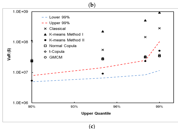
Figure 11. VaR estimates by the classical, DPFS and CPFS methods for the Australian automobile accidents data (a); the US hurricanes loss data (b) and chemical spills data (c). The DPFS Method (I) performs the best in estimating VaR for the automobile accident data, while the GMCM method performs best for the hurricanes data. For the chemical spills data, DPFS Method II performs the best compared to the historical bootstrap VaR while the classical method overestimates the historical VaR and is outside the 99% bootstrap confidence bands.
