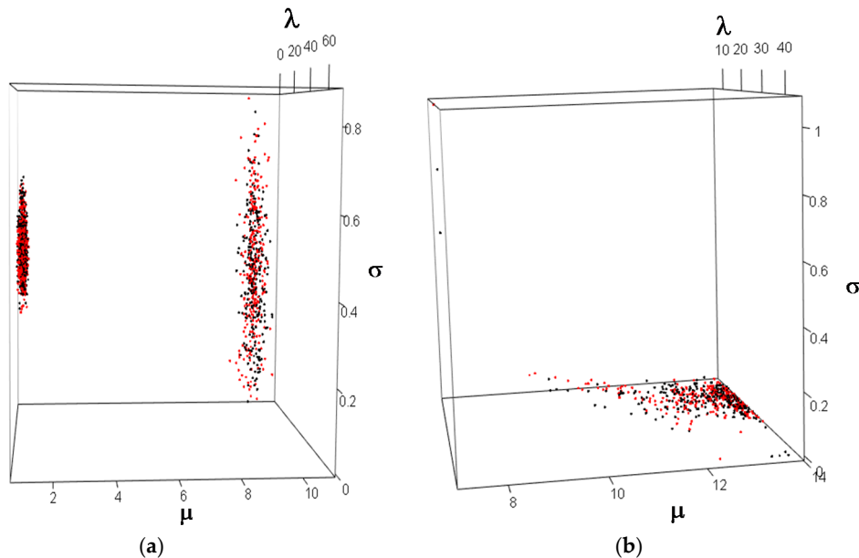
Figure 6. CPFS results: (a) the left panel shows the Gaussian mixture copula model (GMCM) analysis for Scenario (IV); (b) the right panel shows a Gaussian copula analysis for the chemical spills data; red points indicate copula fit, while black are actual data. For both simulated and real-world data, the CPFS method closely fits the real data to the copula function.
