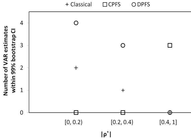
Figure 12. The number of instances when VaR estimation is within 99% bootstrap confidence interval (CI) is plotted versus the magnitude of the correlation ( |\rho^*| ) between loss severity and loss frequency for the three methods; namely, classical, CPFS and DPFS. The number of instances is counted using both simulated and real-world datasets. Examining through all of the data sets, we observe three instances where the CPFS methodology accurately estimates the VaR for all of the upper quantiles of the VaR estimate, namely, 90%, 95%, 98%, 99%, 99.5% and 99.9%. Overall, for |\rho^*| \geq 40\% , the CPFS methodology is the best choice for VaR estimation.
