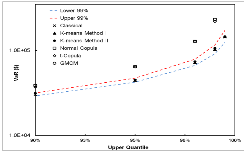
Figure 8. VaR estimates by the classical, DPFS and CPFS methods for the simulated Scenario (III); DPFS Methods (I) and (II) perform comparable to true VaR along with the classical method (since frequency is independent of severity); the copula methods overestimate the VaR in these cases. As seen from this figure, the overlapping points corresponding to the DPFS and classical methods indicate that their respective VaR estimates are within 1% of each other and thus visually indistinguishable.
