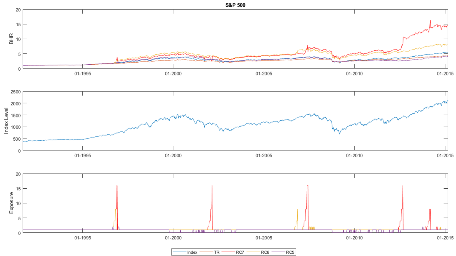
Figure 2. This figure displays the Buy and Hold returns (BHRs) of the volatility-based strategies, the index level and the exposures induced by the trading rule.
