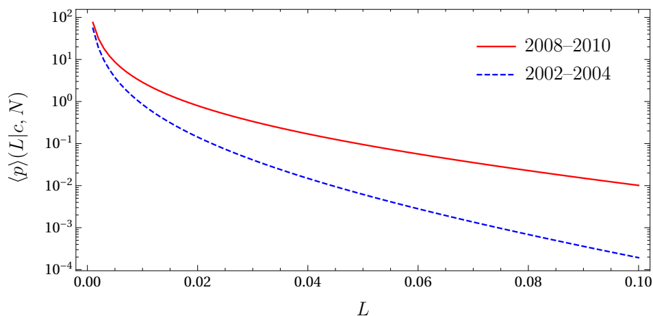
Figure 8. Average loss distribution for different parameters taken from Table 1. The dashed line corresponds to the calm period 2002–2004; the solid line corresponds to the global financial crisis 2008–2010.
