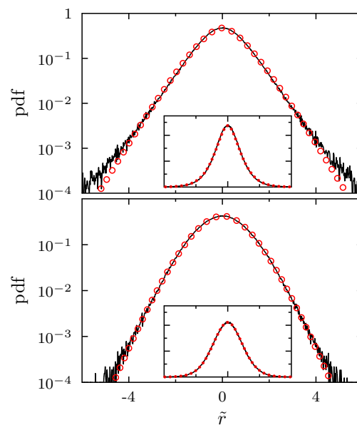
Figure 4. Aggregated distribution of the rotated and scaled returns \tilde{r} for \Delta t = 1 (top) and \Delta t = 20 (bottom) trading days. The circles correspond to the aggregation of the distribution (13). Reproduced with permission from (Schmitt et al. 2013), EPLA.
