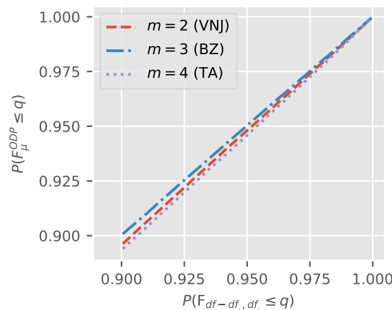
Figure 8. Distribution of F_{\mu}^{ODP} conditional on non-rejection of a 5% Bartlett test.
