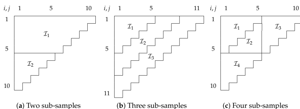
Figure 1. Examples for splits of run-off triangles into two (a), three (b) and four (c) sub-samples. Sub-samples are denoted by \mathcal{I}_\ell . Accident years i are in the rows, development years j in the columns.
