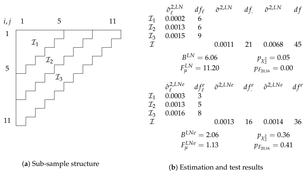
Figure 4. Log-normal chain-ladder (LN) and extended chain-ladder (LNe) model for Barnett and Zehnwirth (2000) data. Sub-sample structure shown in (a), estimation and test results in (b).
