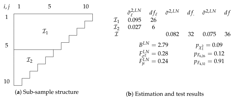
Figure 2. Log-normal chain-ladder model for Verrall et al. (2010) data. Sub-sample structure shown in (a), estimation and test results in (b).
