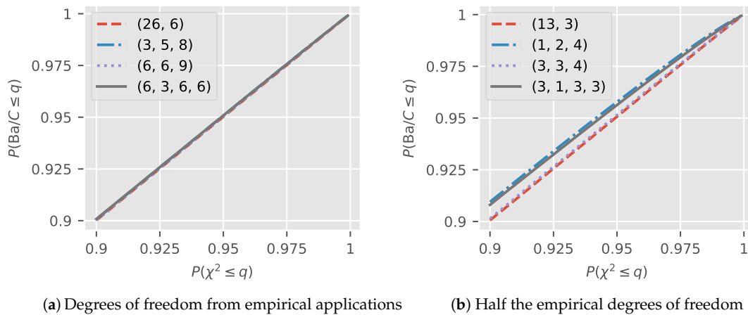
Figure 5. pp-plots for the adjusted Bartlett distribution Ba/C against \chi^2 for varying degrees of freedom. (a) and (b) show results for degrees of freedom corresponding to the empirical applications and half those degrees of freedom, respectively.
