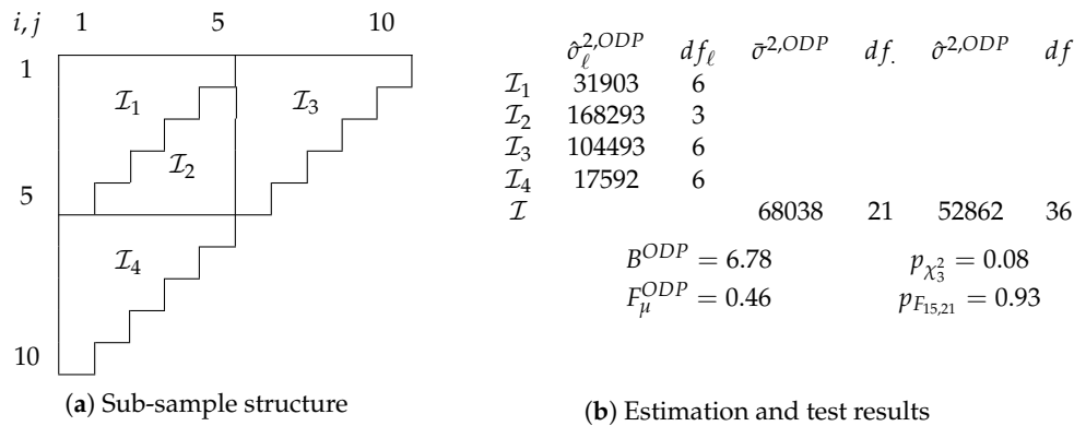
Figure 3. Over-dispersed Poisson chain-ladder model for Taylor and Ashe (1983) data. Sub-sample structure shown in (a), estimation and test results in (b).
