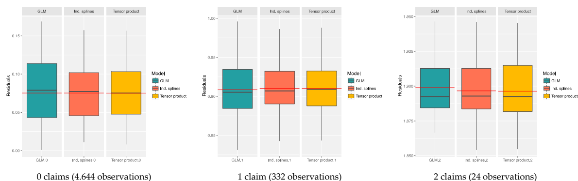
Figure 14. Residuals for insureds with 0, 1 and 2 claims (in each part, left to right GLM, GAM with independent cubic splines and GAM with a tensor product base).
