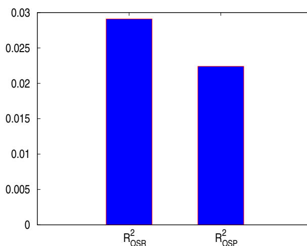
Figure 4. The R_{OSP}^2 , and R_{OSR}^2 of S&P 500 monthly prices from December 2011 to November 2016.
