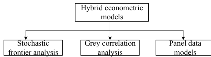
Figure 2. Construction of hybrid econometric models.
