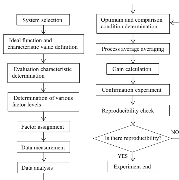
Fig. 8 Robust design procedure
