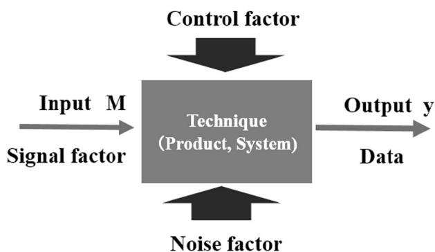
Fig. 7 Robust design
