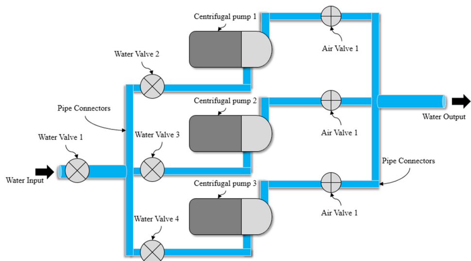
Fig. 4 The centrifugal pumping 2-out-of-3 redundant system
