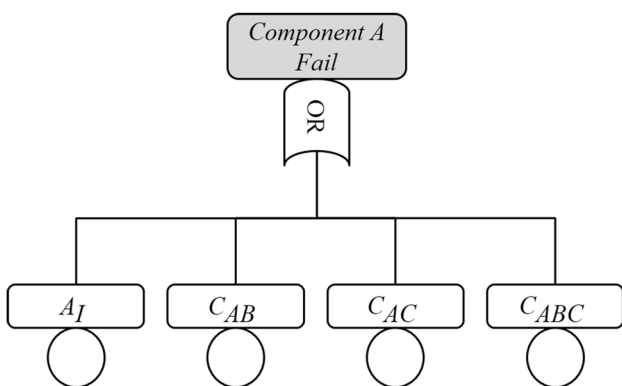
Fig. 2 The fault tree of component A
