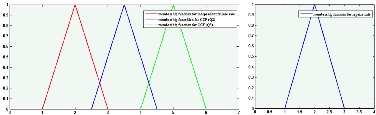
Fig. 3 The membership function for failure rates and repair rate
