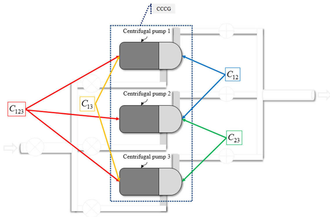
Fig. 5 CCCG for centrifugal pumping 2-out-of-3 redundant system
