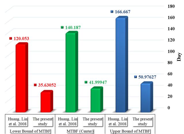
Fig. 7 The comparison of MTBF for the two models
