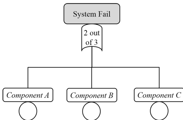
Fig. 1 The fault tree of 2-out-of-3 redundant system
