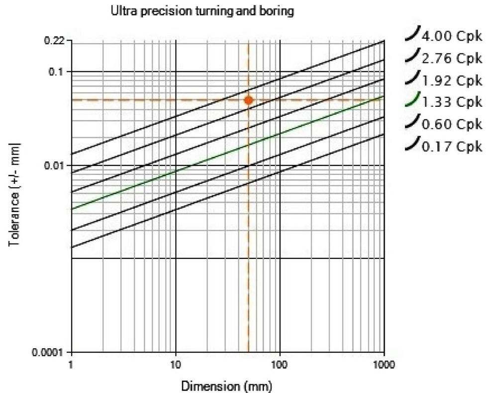
Fig. 9 Graphical plot for center hole diameter precision boring with predicted C_{pk} of 3.27 for predetermined tolerance of \pm 0.050 mm
