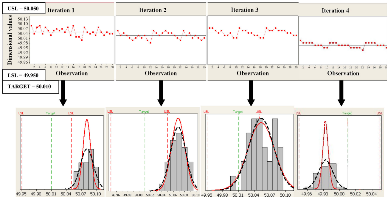
Fig. 6 Process capability analysis depicting run charts and histograms of Iterations 1, 2, 3 and 4
