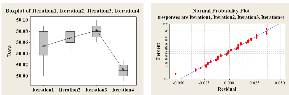
Fig. 11 The box plot and normal probability plot for center bore hole dimensional observations
