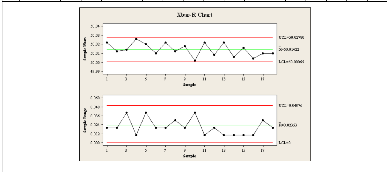
Fig. 8 \bar{X} and R control chart
