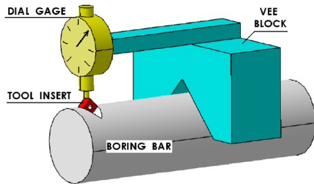
Fig. 7 Schematic diagram of tool insert setting Vee-Block
