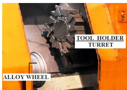
Fig. 4 Set up for center bore diameter machining operation
