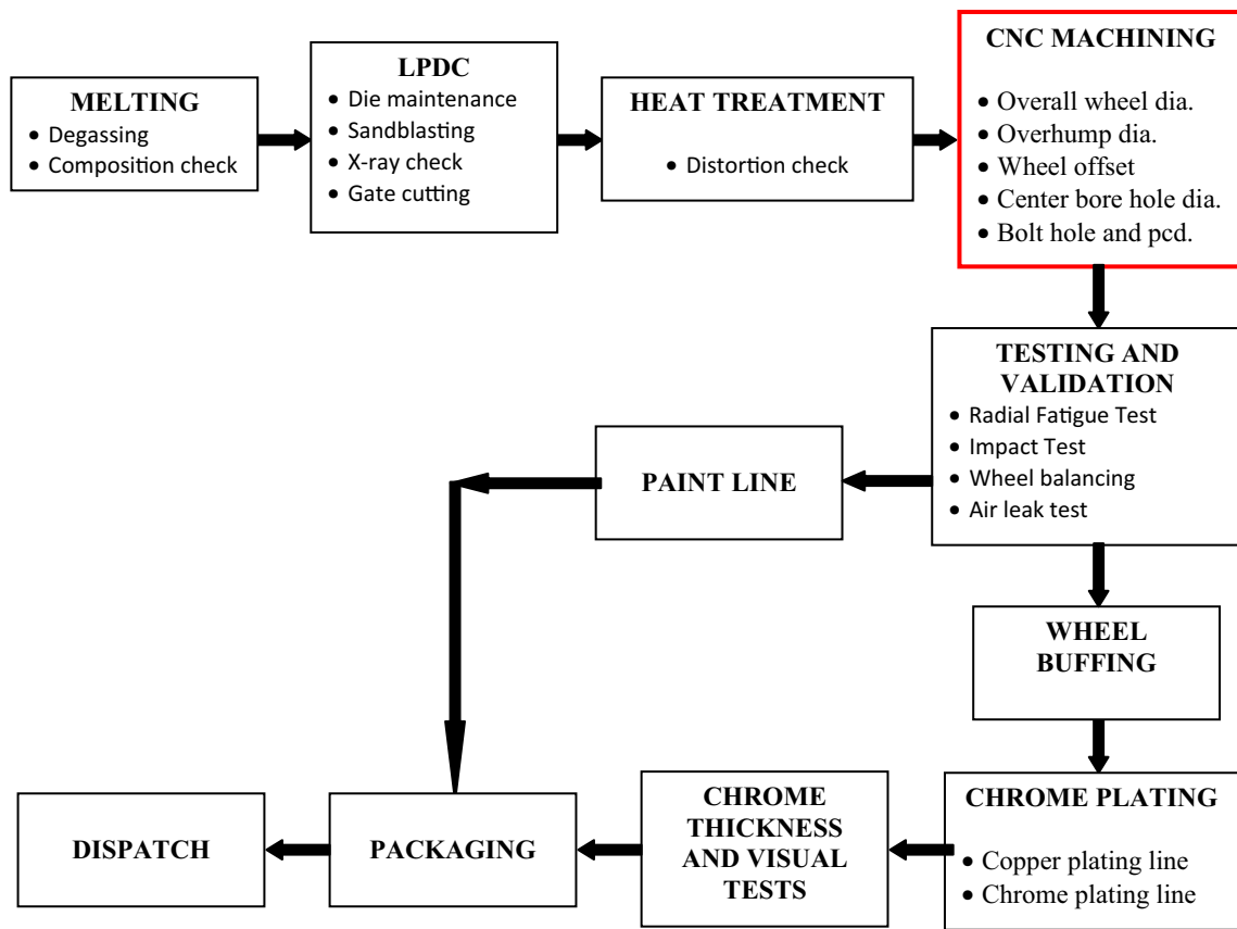
Fig. 1 Process flow chart of A356 aluminum alloy wheel manufacturing process
