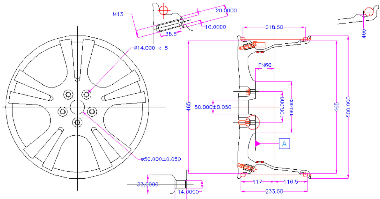
Fig. 2 Alloy wheel machining drawing with center hole diameter of \phi 50.000^{(\pm 0.050)}
