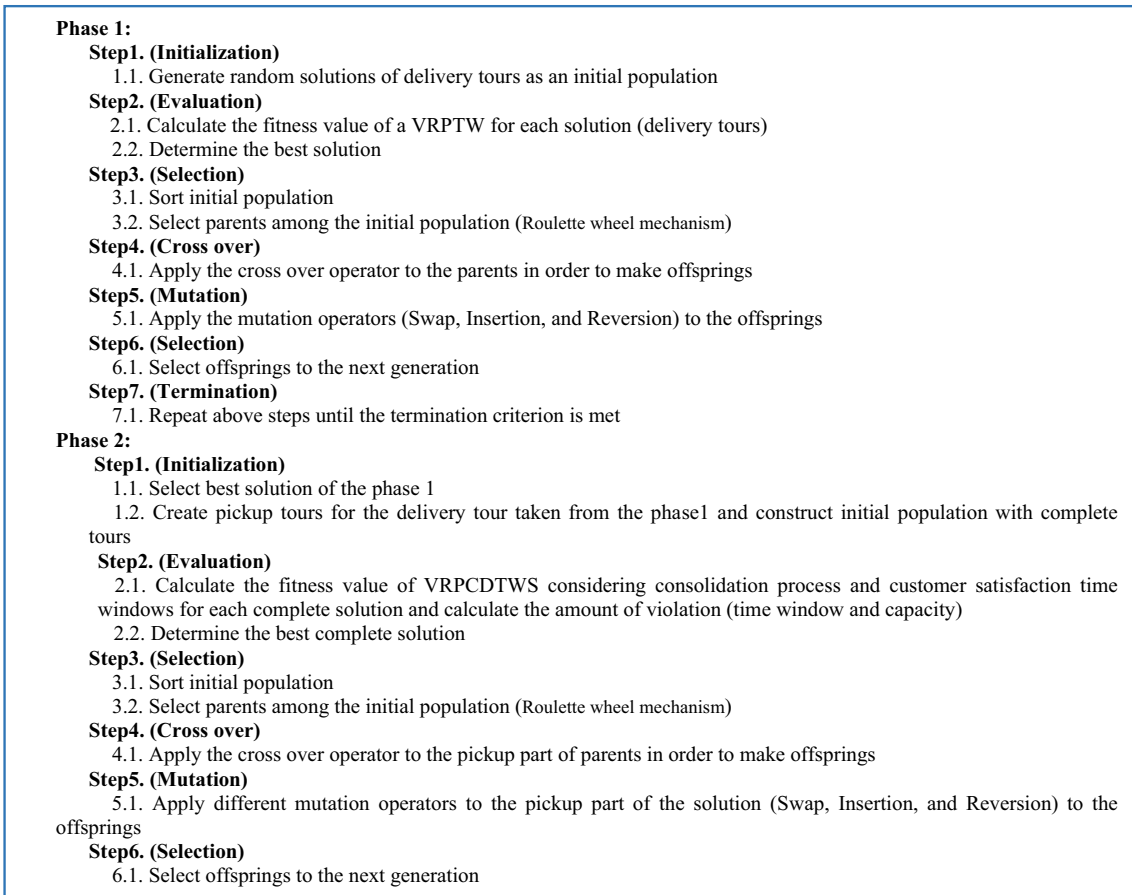
Fig. 7 Proposed two phase GA structure
