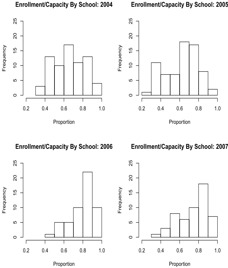
FIGURE 2. School capacity: 2004-2007
