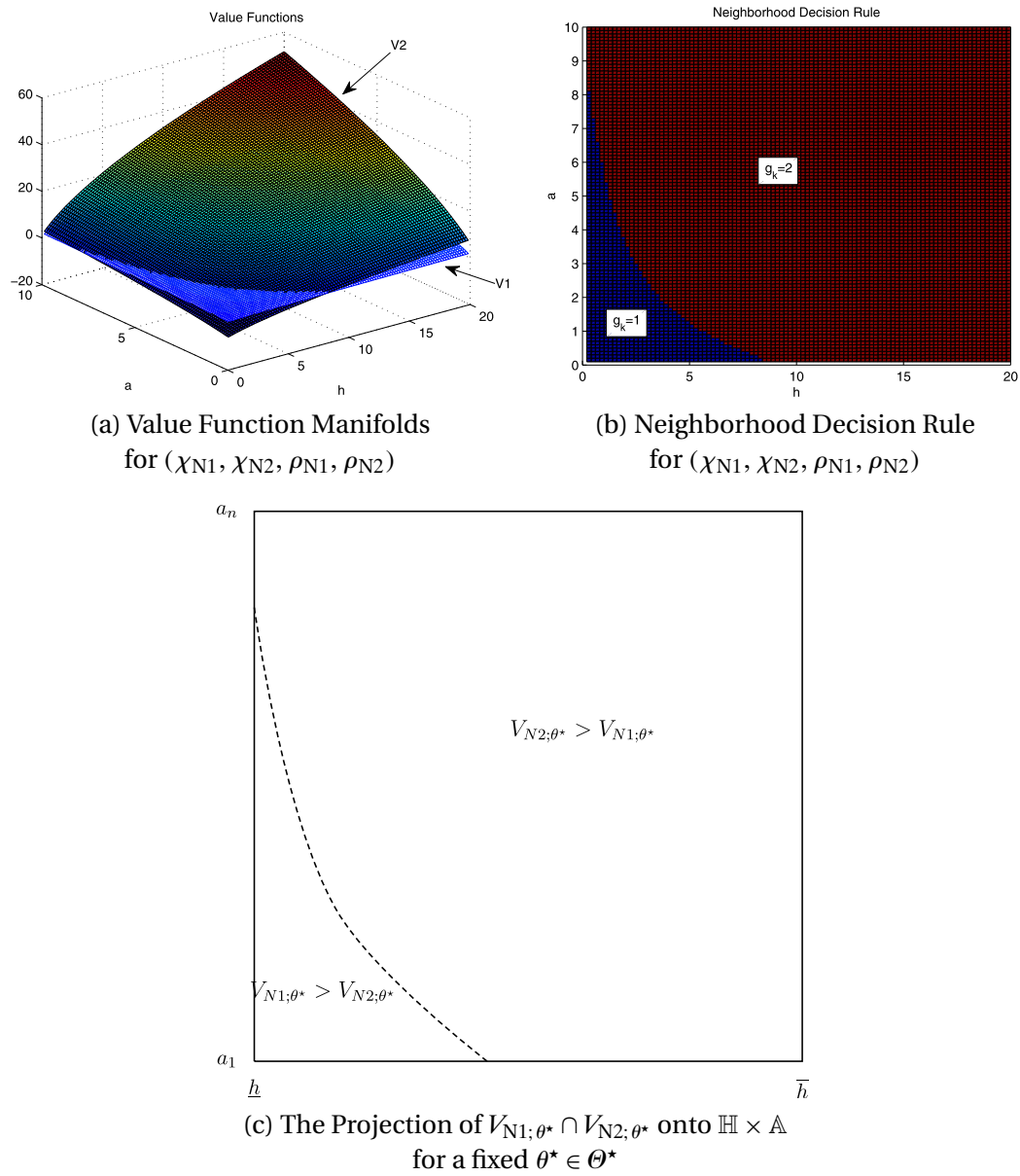
FIGURE 21. Value functions for parameters (\chi_{N1}, \chi_{N2}, \rho_{N1}, \rho_{N2}) likely to be in \Theta^* .
