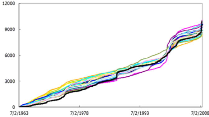
FIGURE 5. Quadratic variations of market return and fitted residuals. Notes: There are 26 lines in the figure. The thick darker line represents the quadratic variation series, estimated by the realized variance series, of the daily excess market returns, and the remaining 25 lines represent the quadratic variation series of the 25 fitted residuals from Fama–French three-factor regression on 25 portfolios sorted by 5 size and 5 B/M ratio groups.
