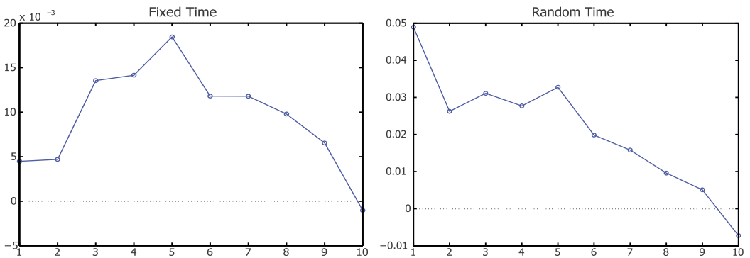
FIGURE 9. Alphas of size portfolios.
