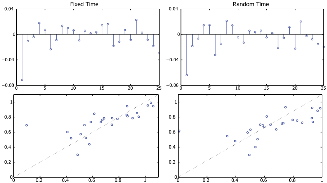
FIGURE 12. Fama–French alphas and betas of (size, B/M) portfolios. Notes: The left panels display alphas (top) and betas (bottom) estimated from the fixed time regression, while the right panels present those from our random time regression. The betas here represent the predicted returns from Fama–French regressions and are plotted along with the average excess returns for each portfolio, following Cochrane (2001, p. 441).
