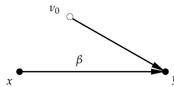
Figure 1. Graph of the structural relationship (11).
