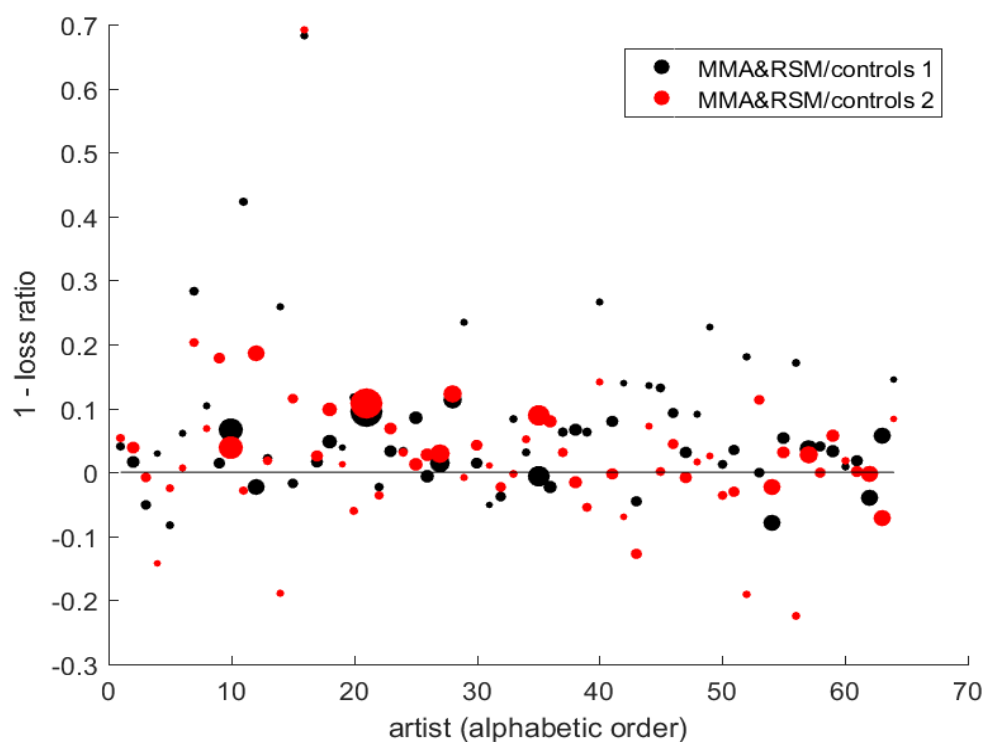
Figure 2. Reduction in RMSE from model-average+ RSM relative to simple hedonic model. (The figure displays [1 - \text{RMSE}(\text{combined model average} + \text{RSM})/\text{RMSE}(\text{hedonic model})] for the 64 artists named in Appendix A. Positive values therefore indicate reduced loss (superior performance) of the model average, with repeat sales where available, relative to the single OLS hedonic model for a particular artist. Model 1 is the hedonic regression with selected dummies + painting dimensions, surface area, age of artist at time of execution, and age squared. Model 2 is the same without dummies. The sizes of dots are proportional to total sample sizes for the artist.)
