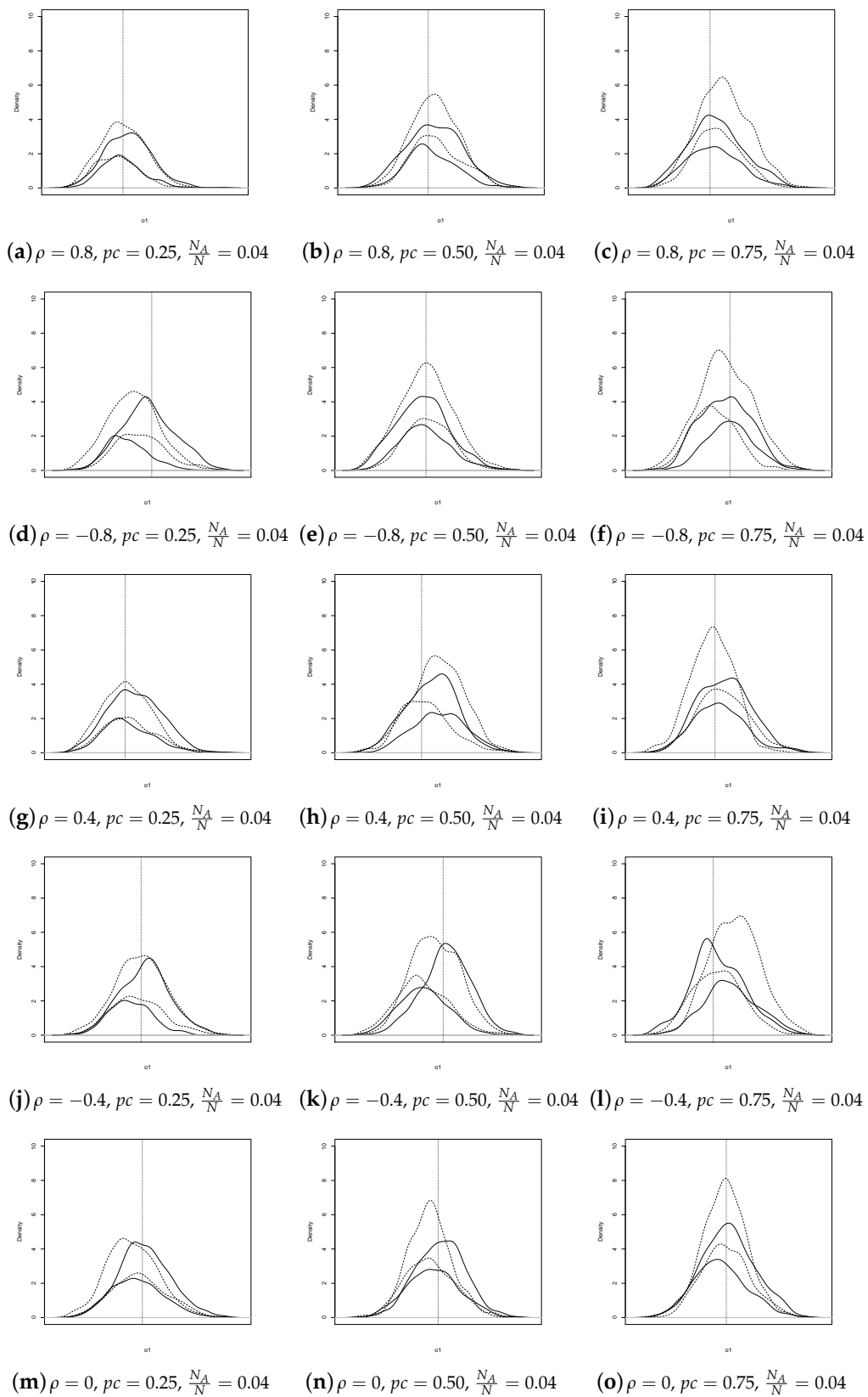
Figure 1. Densities of \hat{\beta}_1 for some values of \rho , N_A/N = 0.04 and three sampling proportions of cases pc (SRS: dashed lines; GE: continuous line; n = 2000 for the two flatter distributions; n = 10,000 for the two more sharpened distributions).
