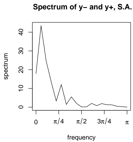
Figure 3. Spectra of y_t^- and y_t^+ seasonally adjusted.
