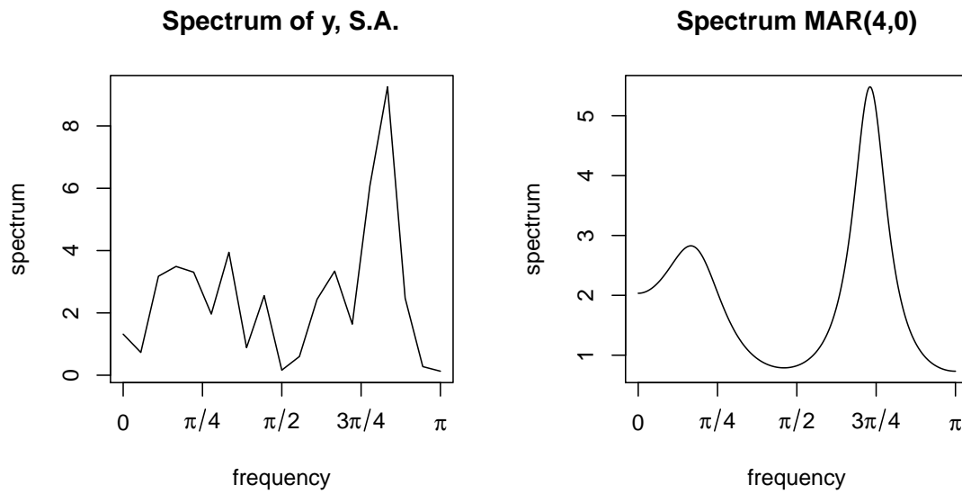
Figure 2. Spectra of y_t seasonally adjusted (left) and an MAR(4,0) process (right).
