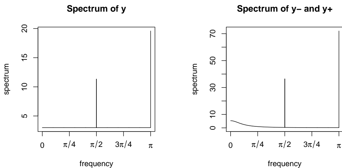
Figure 1. Spectra of data generating processes y_t (left), y_t^- and y_t^+ (right).
