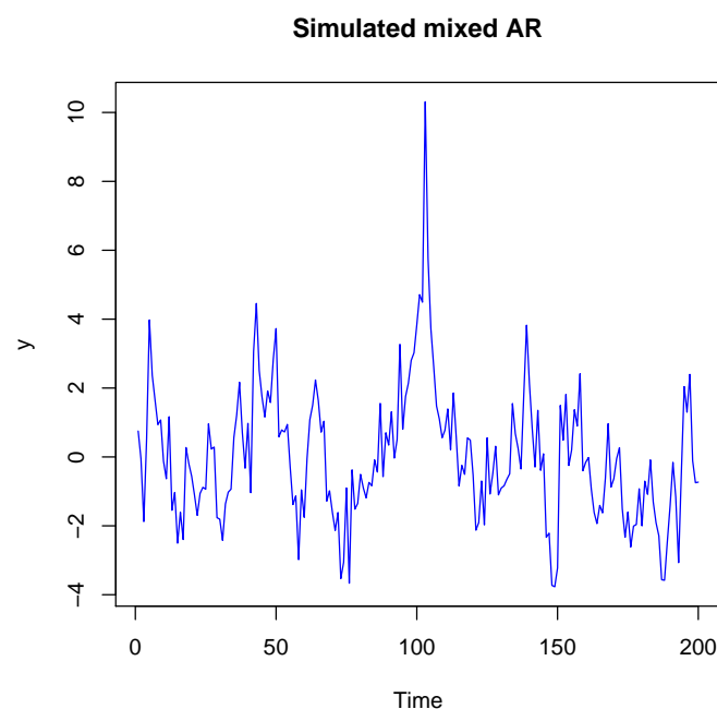
Figure 4. Simulated MAR(2,2) process with \phi = [0.2, 0.3]' , \varphi = [0.3, 0.1]' , \epsilon_t \sim t_5 .
