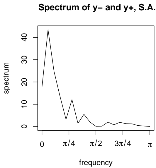
Figure 3. Spectra of y_t^- and y_t^+ seasonally adjusted.
