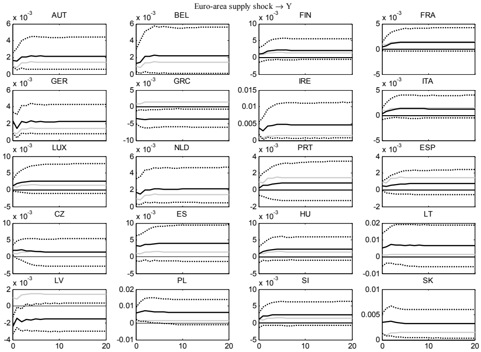
Figure 6: Impulse responses of output and inflation of individual countries (black) and euro-area aggregates (gray) to euro-area shocks 1)
