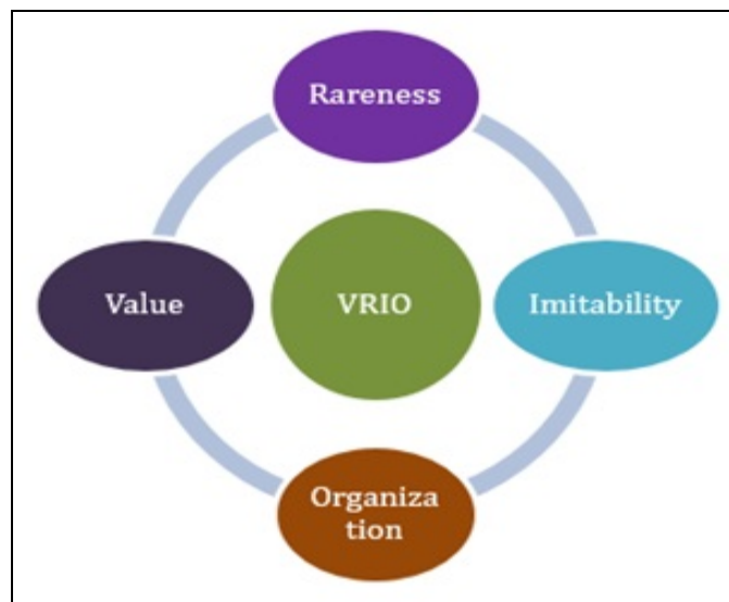
Figure 2: VRIO Model
