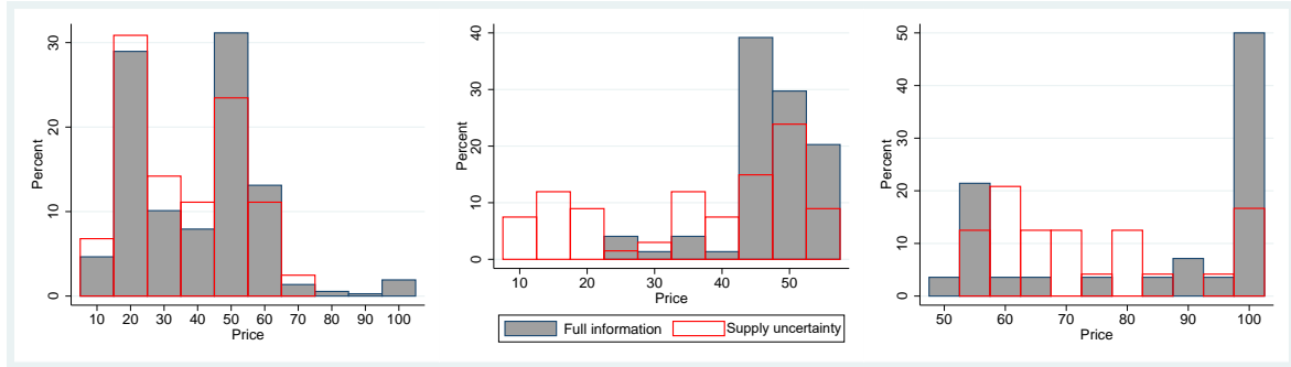
Figure 4: Supply uncertainty effects
