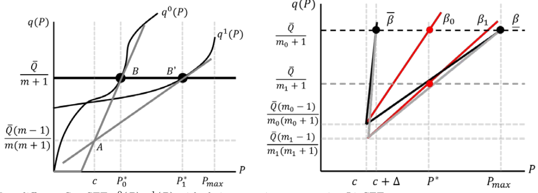
LEFT: Two different SymSFE q^0(P), q^1(P) with their two unique supporting LinSFE. RIGHT: The black and gray lines depict the range of all LinSFE for two different levels of competition ( m_1 > m_0 \geq 1 ) using the bounds in (6). Red lines: Obtaining the price P^* under m_1 requires more bid shading than under m_0 ( \beta_1 < \beta_0 ).
