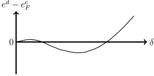
(c) \omega = 0.41 : \underline{\delta}(\omega) > 0 , \bar{\delta}(\omega) > 0 .
