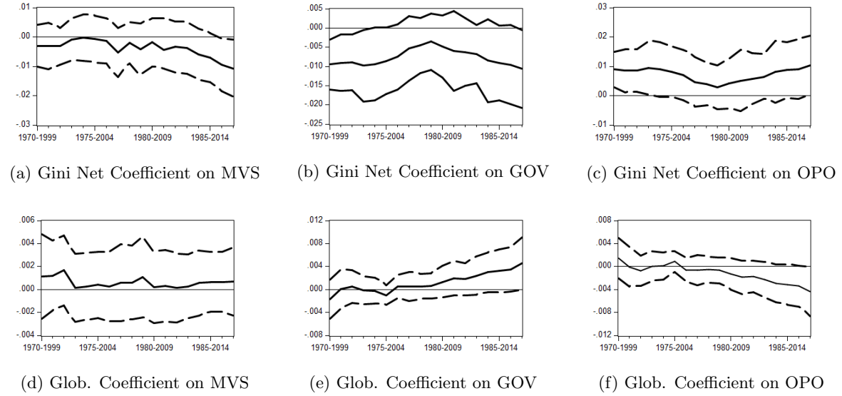
Figure 4: Time-varying coefficients (not standardized) obtained from rolling panel regressions of MVS, GOV and OPO.
