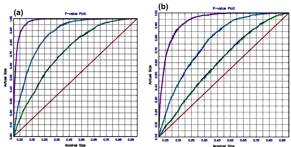
Figure 2. Power of the unit root tests of Model 1 for 500 observations with white noise: (a) Model 1 and (b) Model 2.
