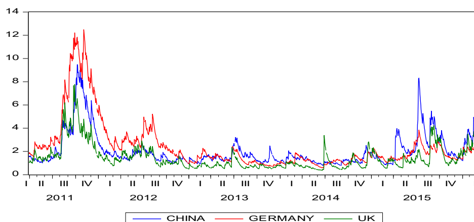
Figure 4. Variances of ETF returns: China, Germany and UK.
