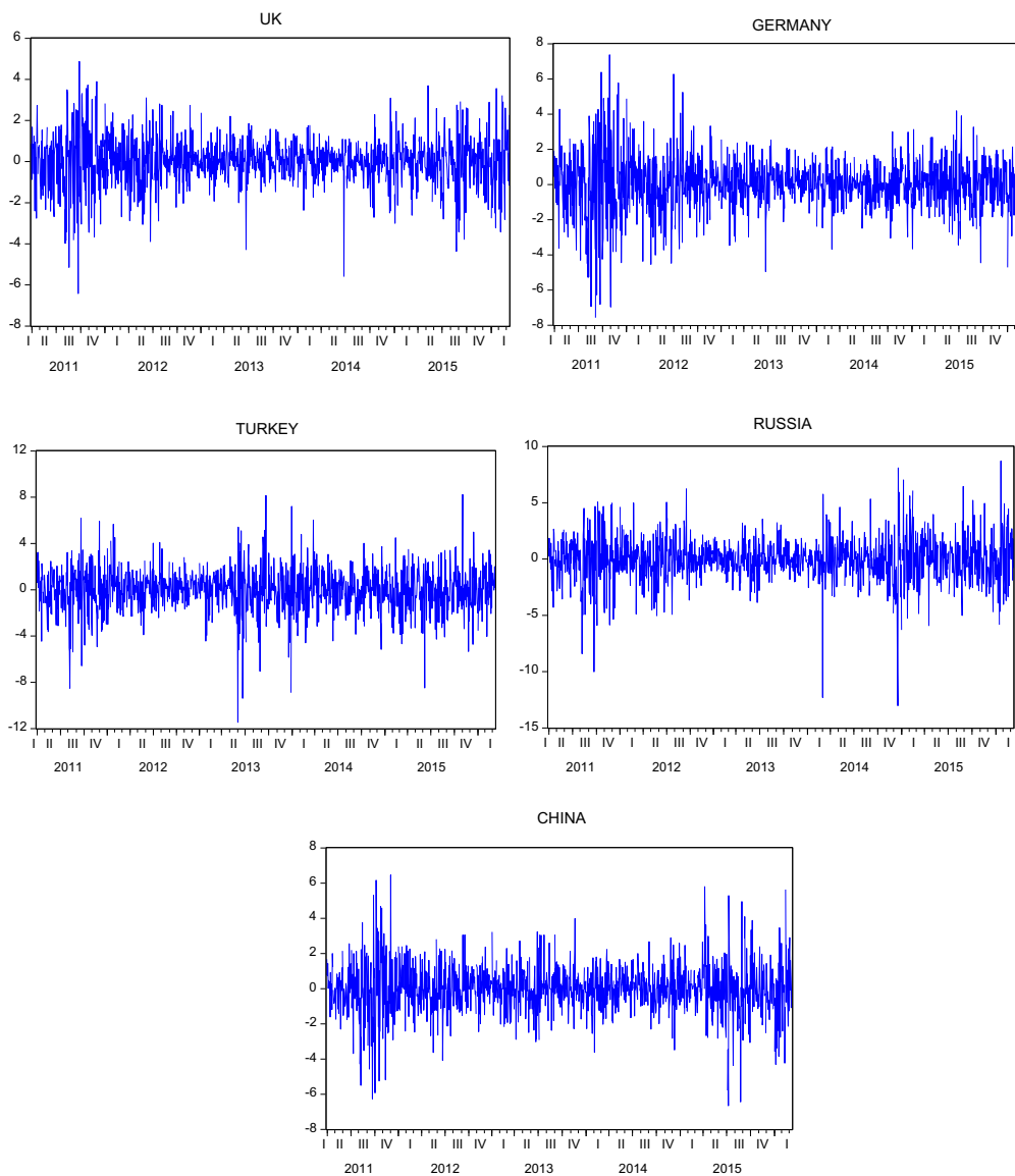
Figure 1. Graphs of daily returns of selected ETFs.
