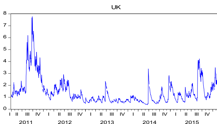
Figure 2. GARCH graph of ETF returns for UK
