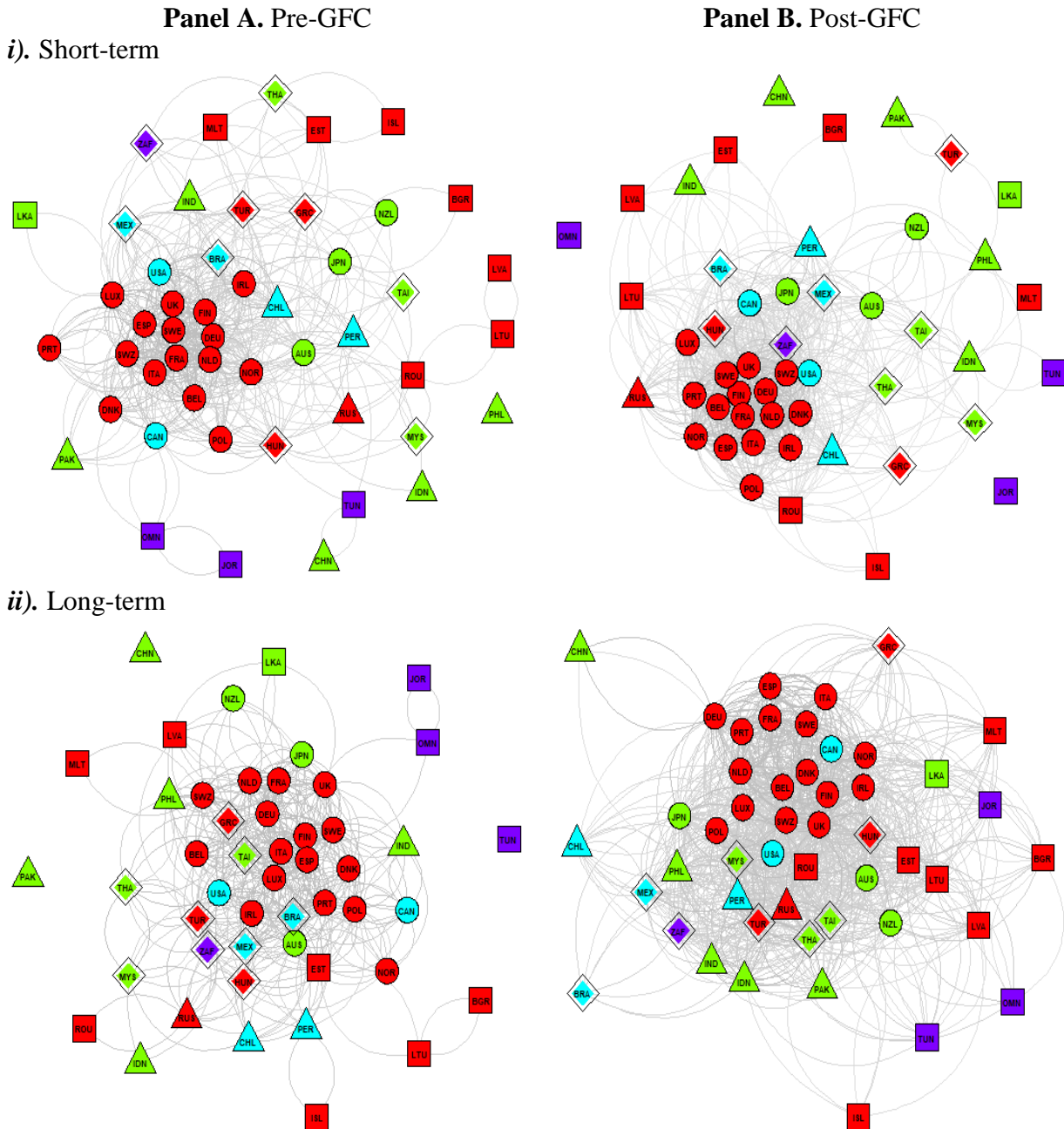
Figure 2. Quantile coherency network – Bullish market conditions (percentile 0.95)
