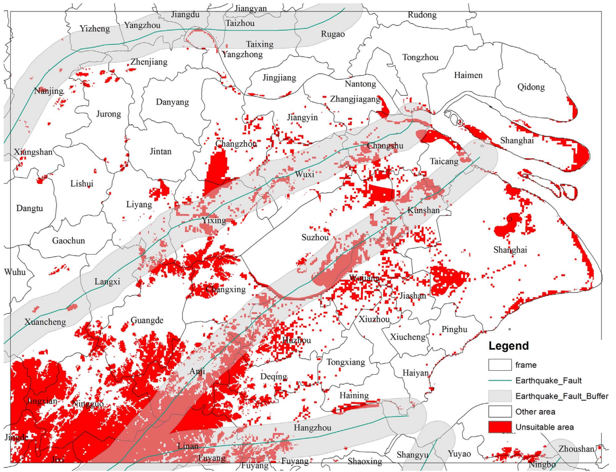
Fig. 4. Environmentally unsuitable area for urban development in the Changjiang Delta Region, 2010.
