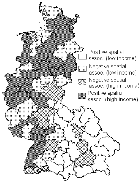
Fig. 1. Spatial association of \ln(y_{76})
