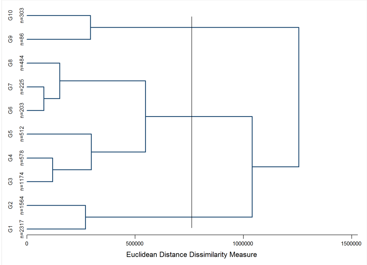
Figure 1: Dendrogram of Ward's method.
