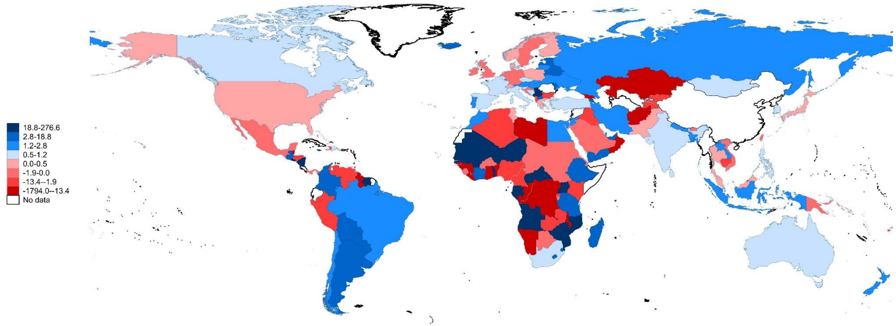
Model IV-2nd, period 2002-2015
