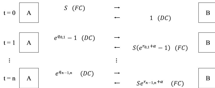
Figure 4: Cash flows of an n -period CCBS
