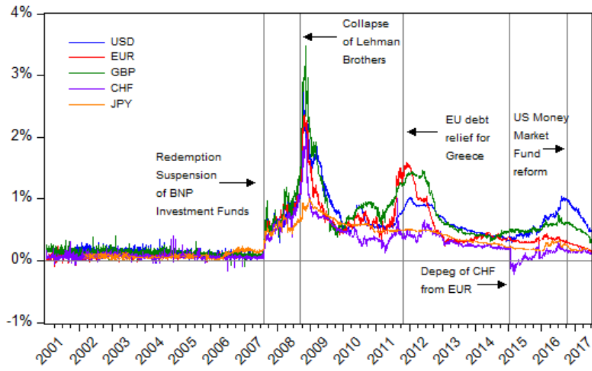
Figure 1: 12-month Libor-OIS spreads of major currencies
