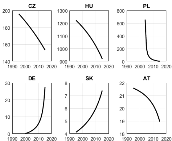
Figure 4 Time series of MRTS calculated for each country during the period under observation ( MRTS on the vertical axis, time t on the horizontal axis).
