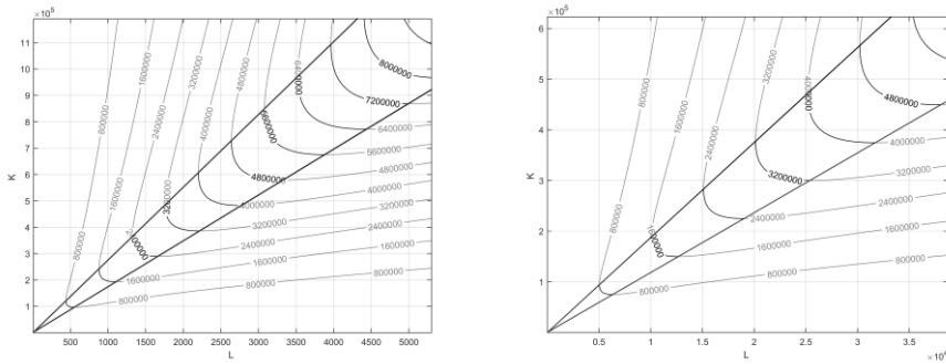
Figure 2 Isoquant maps based on the parameters estimated via NLS for the year 2005; the Czech Republic on the left-hand side, Germany on the right-hand side.
