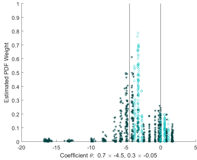
(b) Estimated pdf for \theta
