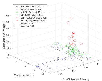
(e) Model IV \tau Heterogeneous; f(\eta, m)
