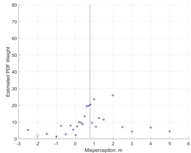
(f) Model IV \tau Heterogeneous; f(m)
