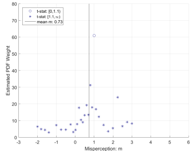
(b) Model II Smaller Span; f(m)
