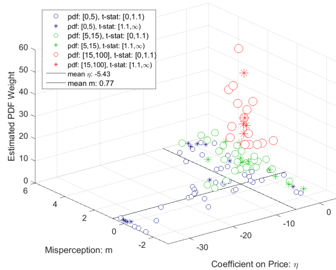
FIGURE 2. Joint Probability Distribution for \eta and m
