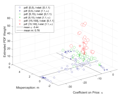
(c) Model III Dense Grid; f(\eta, m)
