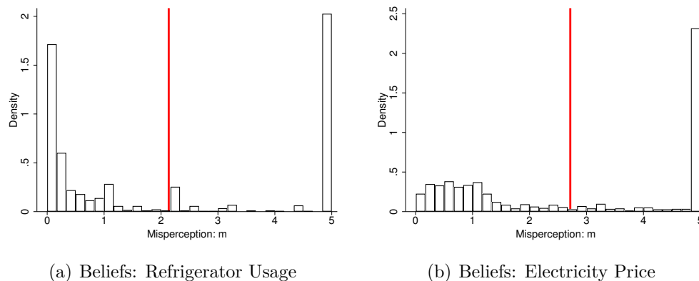
FIGURE 3. Beliefs Valuation Ratios: Refrigerator Usage and Electricity Price
