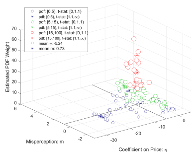
(a) Model II Smaller Span; f(\eta, m)
