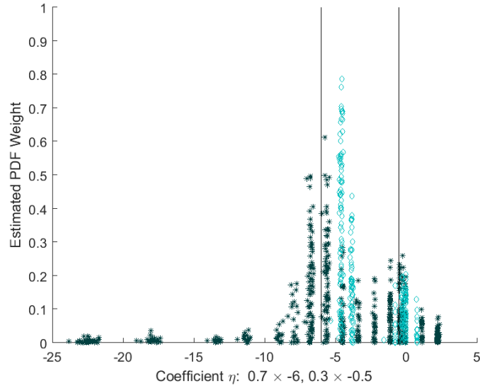
(a) Estimated pdf for \eta
