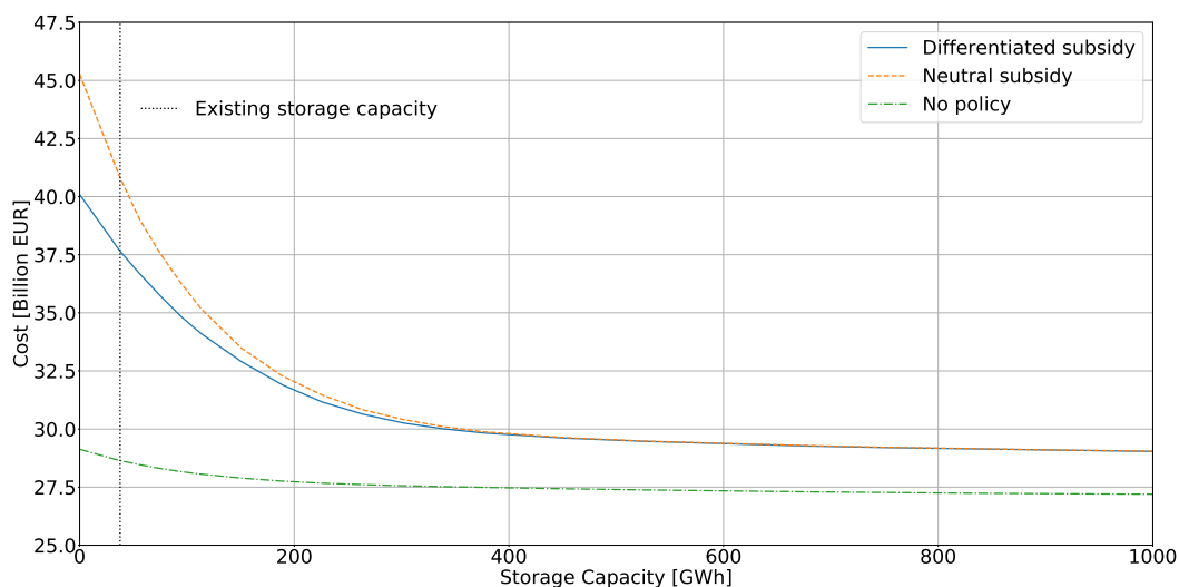
Figure 3: Total cost for rising storage capacity.
