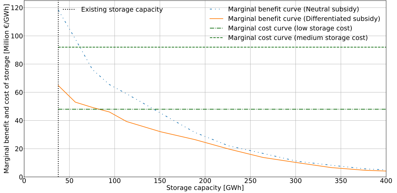
Figure 7: Marginal costs and benefits for different levels of energy storage and technology-neutral and technology-specific RE support schemes.
