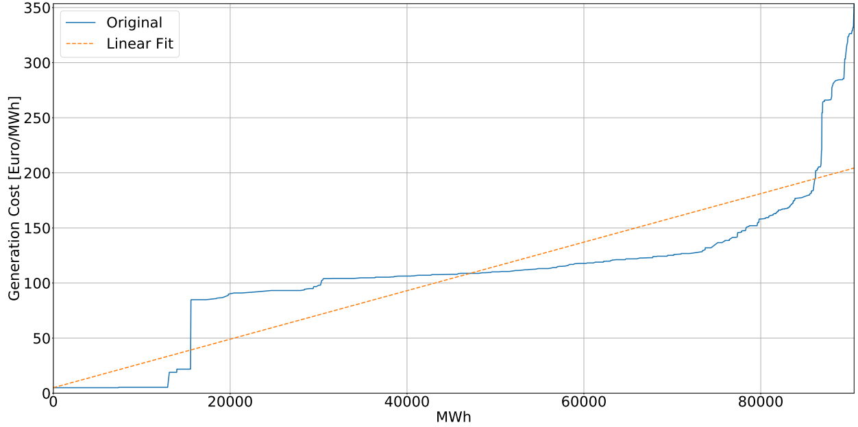
Figure 2: Linear fit to merit order of marginal generation cost of conventional electricity producers in Germany. The linear fit is used as supply curve for conventionals in the simulations of section 4.
