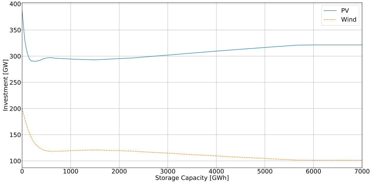
Figure 4: RE investment with increasing storage capacity.
