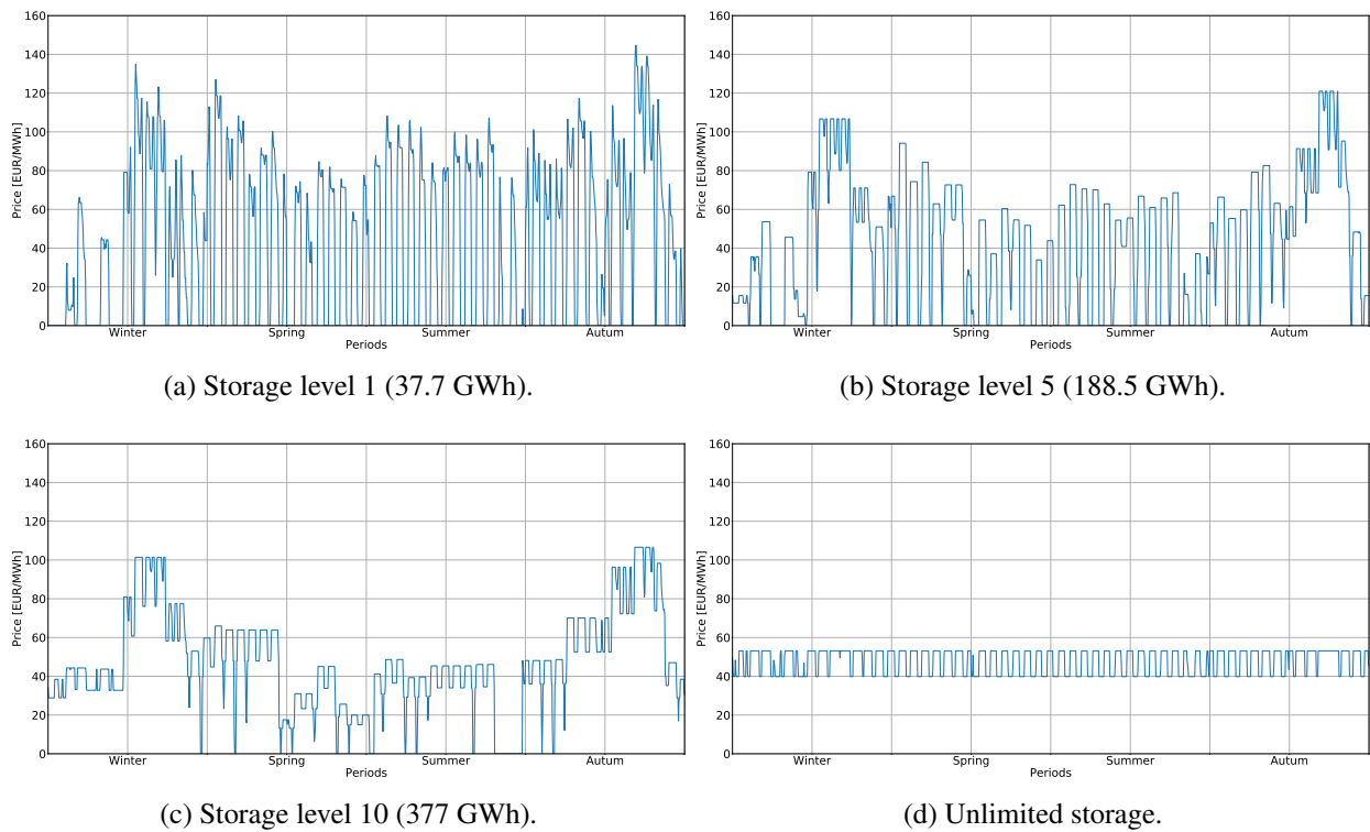
Figure 5: Hourly electricity price for a 70% RE target with a technology-neutral RE subsidy and increasing storage capacity measured in multiples of the currently (i.e., year 2014) installed level.
