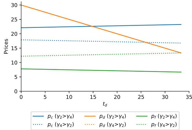
Figure 19: Effect on the prices of EVs, GVs and EVCSs when a subsidy to EVCSs applies, with the model parameters \gamma_1 = 0.4, \gamma_2, \gamma_4 \in \{0.4, 0.6\}, \alpha_c = 40, \alpha_d = 60, \alpha_f = 20, c_c = 0, c_d = 0 and c_f = 0 .
