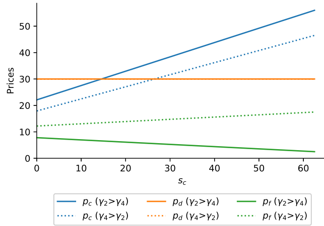
Figure 18: Effect on the prices of EVs, GVs and EVCSs when a tax on GVs applies, with the model parameters \gamma_1 = 0.4, \gamma_2, \gamma_4 \in \{0.4, 0.6\}, \alpha_c = 40, \alpha_d = 60, \alpha_f = 20, c_c = 0, c_d = 0 and c_f = 0 .
