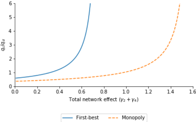
Figure 2: Ratio of EVs to GVs in first-best and monopoly as a function of total network effects.
