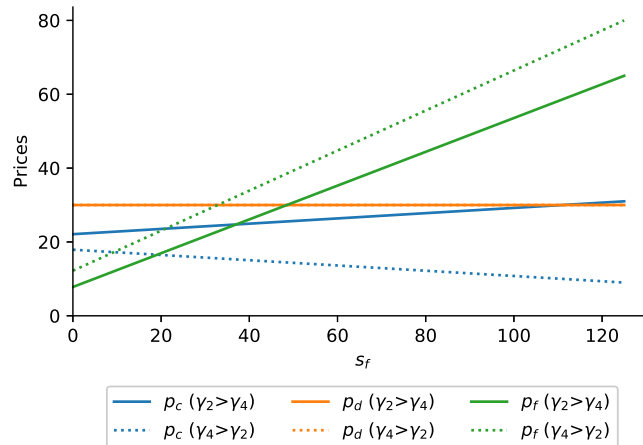
Figure 19: Effect on the prices of EVs, GVs and EVCSs when a subsidy to EVCSs applies, with the model parameters \gamma_1 = 0.4, \gamma_2, \gamma_4 \in \{0.4, 0.6\}, \alpha_c = 40, \alpha_d = 60, \alpha_f = 20, c_c = 0, c_d = 0 and c_f = 0 .
