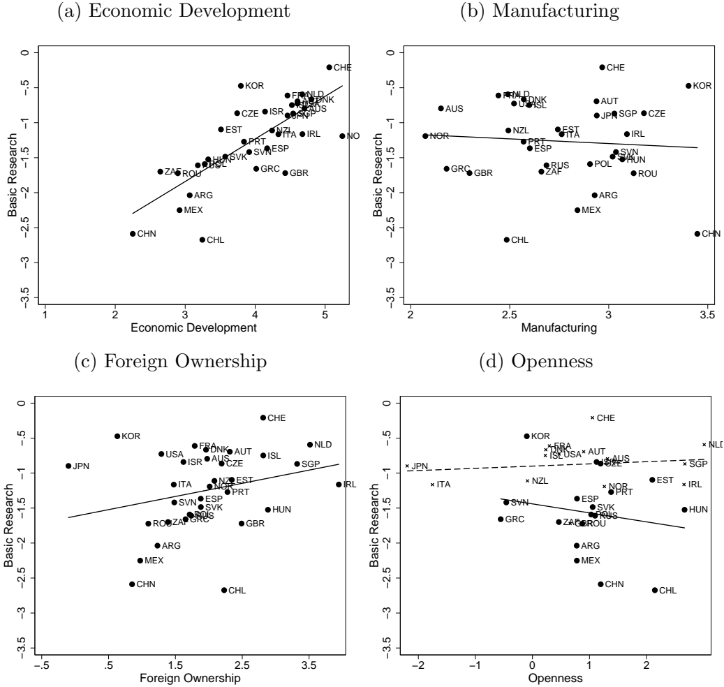
Figure 5: Correlations
