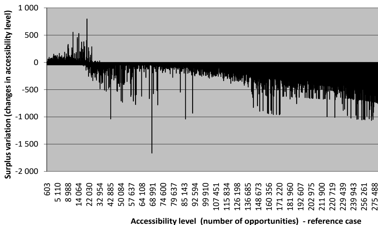
Figure 15. Surplus variation according to the starting accessibility level (zone toll)
