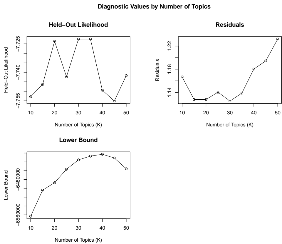
Figure 18: Results of “SearchK” function (stm package)
