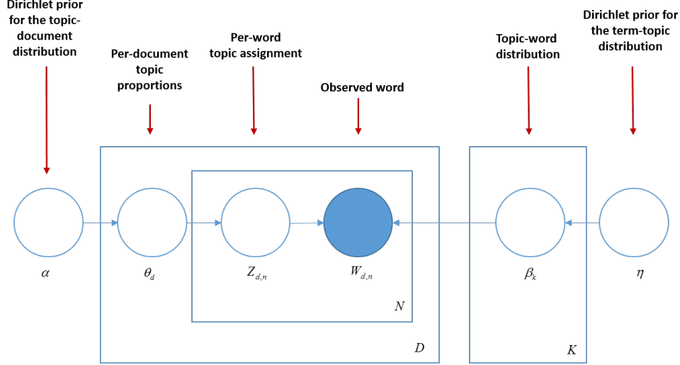
Figure 1: Model Representation of LDA
