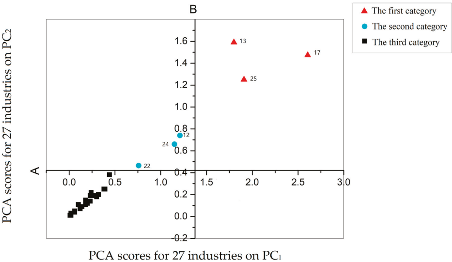
Figure 4. Principal component analysis.
