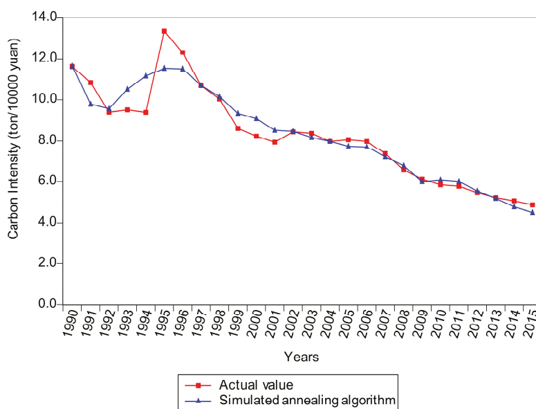
Figure 4. Fitting chart of the carbon intensity prediction model.
