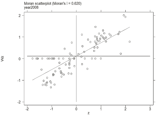
Figure 3. The local Moran index in 2008.
