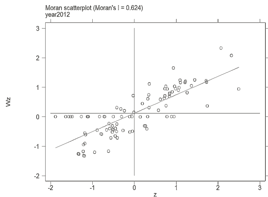
Figure 4. The local Moran index in 2012.
