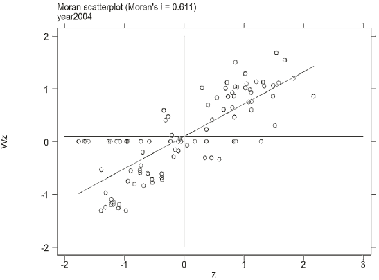
Figure 2. The local Moran index in 2004.
