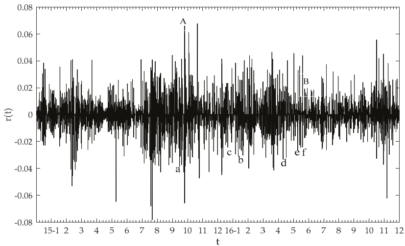
Figure 1. Logarithmic returns of fuel oil futures.
