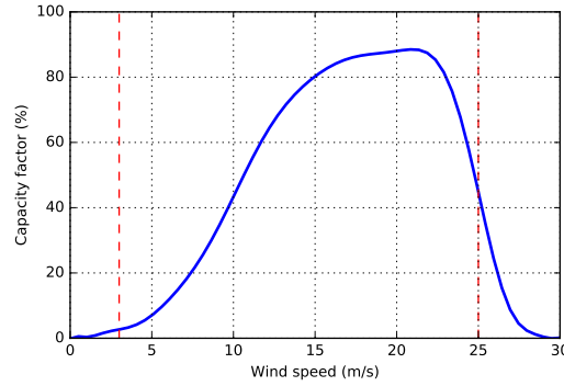
Figure 2: Wind speed to capacity factor curve (Ofgem, 2013).
