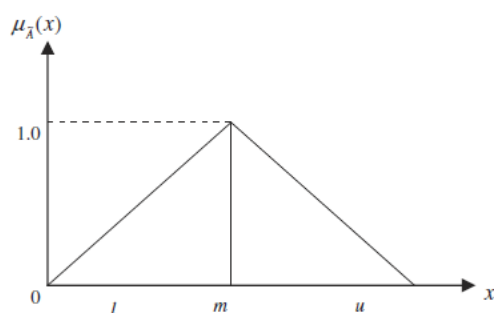
Figure 1. Membership functions of triangular fuzzy numbers
