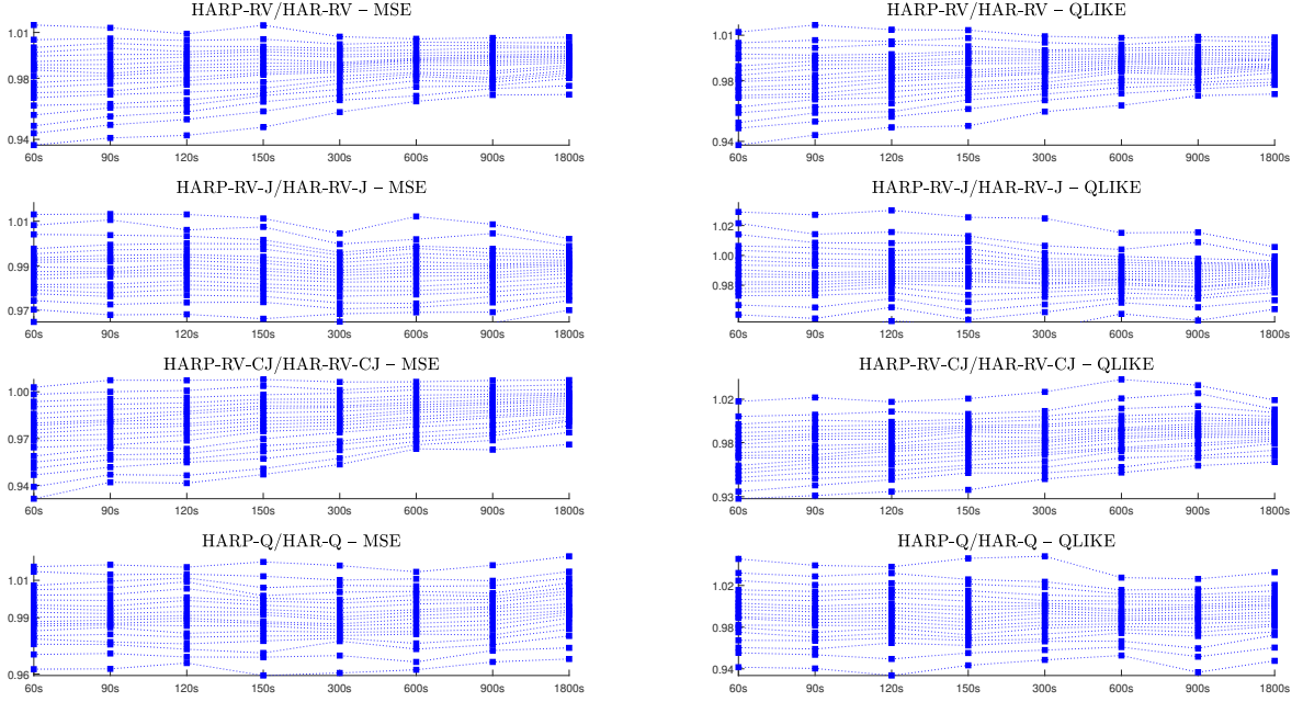
Figure 6: Loss ratio for simulated data – h = 5
