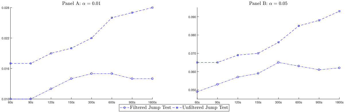
Figure 4: Proportion of spurious jumps by sampling frequency for filtered and unfiltered data
