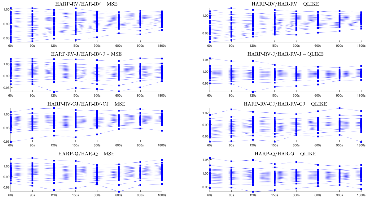
Figure 5: Loss ratio for simulated data – h = 1
