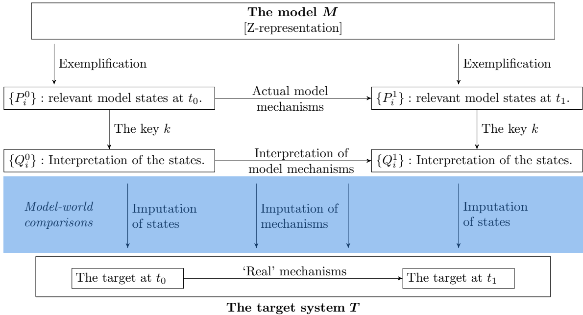
Figure 1: A visualization of the DEKI framework. Note that the denotation of from the model to the target is not visualized for reasons of readability.
