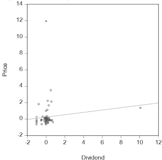
Figure 5. Scatter diagram of dividend versus stock price
