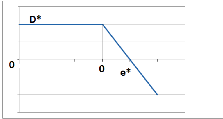
Figure 5: \theta^U - LATE as a function of \varepsilon
