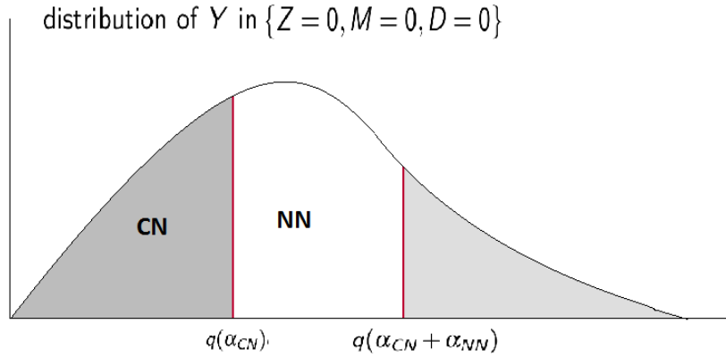
Figure 4: Unconstrained lower bound \mathbb{E}^L[Y(0,0)|CN]
