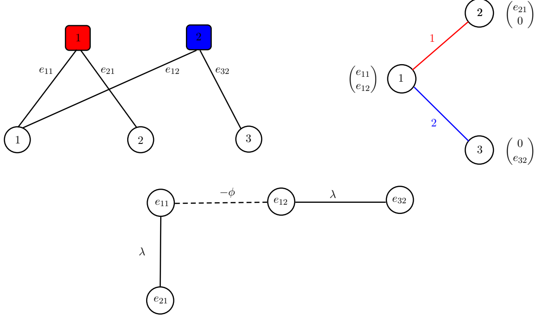
Figure 1: (Top left panel) The bipartite collaboration network \mathcal{G} of authors and projects analyzed in Example 1, where circles represent authors and squares represent projects. (Top right panel) The projection of the bipartite network \mathcal{G} on the set of coauthors. The effort levels of the individual agents for each project they are involved in are indicated next to the nodes. (Bottom panel) The line graph L(\mathcal{G}) associated with the collaboration network \mathcal{G} , in which each node represents the effort an author invests into different projects. Solid lines indicate nodes sharing a project while dashed lines indicate nodes with the same author.
