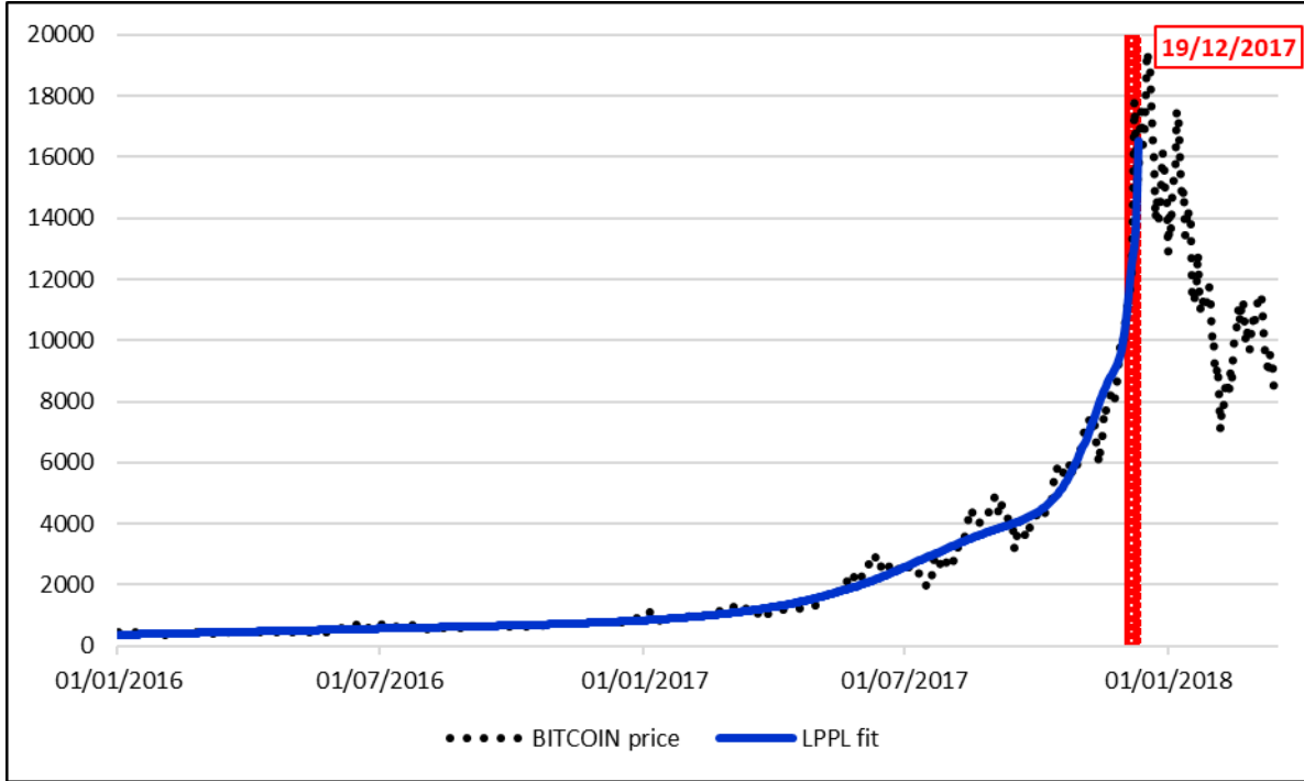
Figure 9. LPPL fit for BTC (model with the minimum RMSE)
