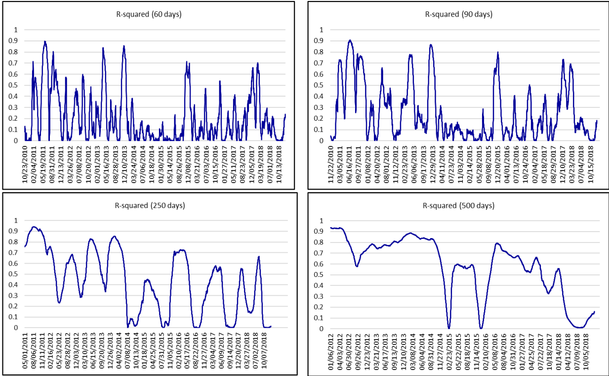
Figure 6. Adjusted R-squared for the Metcalfe's law (equation 5), estimated on rolling windows of 60, 90, 250 and 500 trading days
