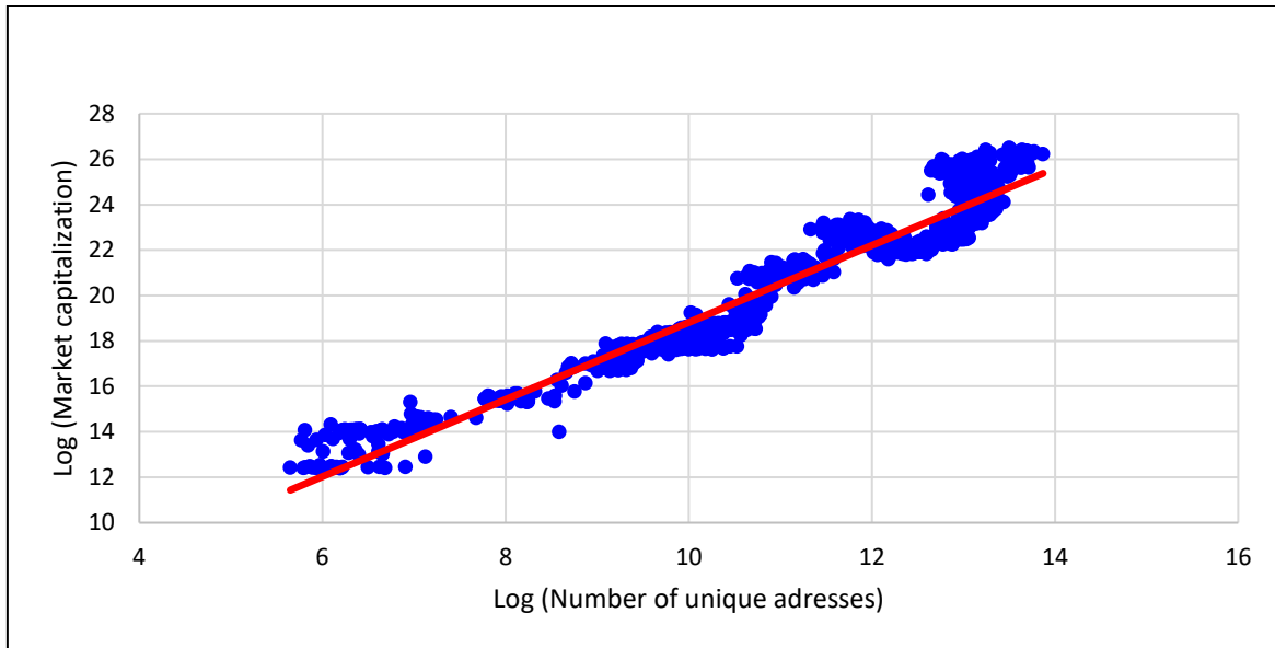
Figure 4. Generalised Metcalfe’s law for Bitcoin’s market capitalization, for the entire data sample
