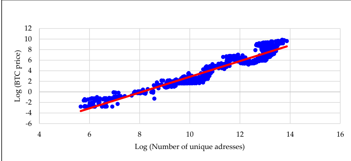
Figure 5. Generalised Metcalfe’s law for Bitcoin’s price
