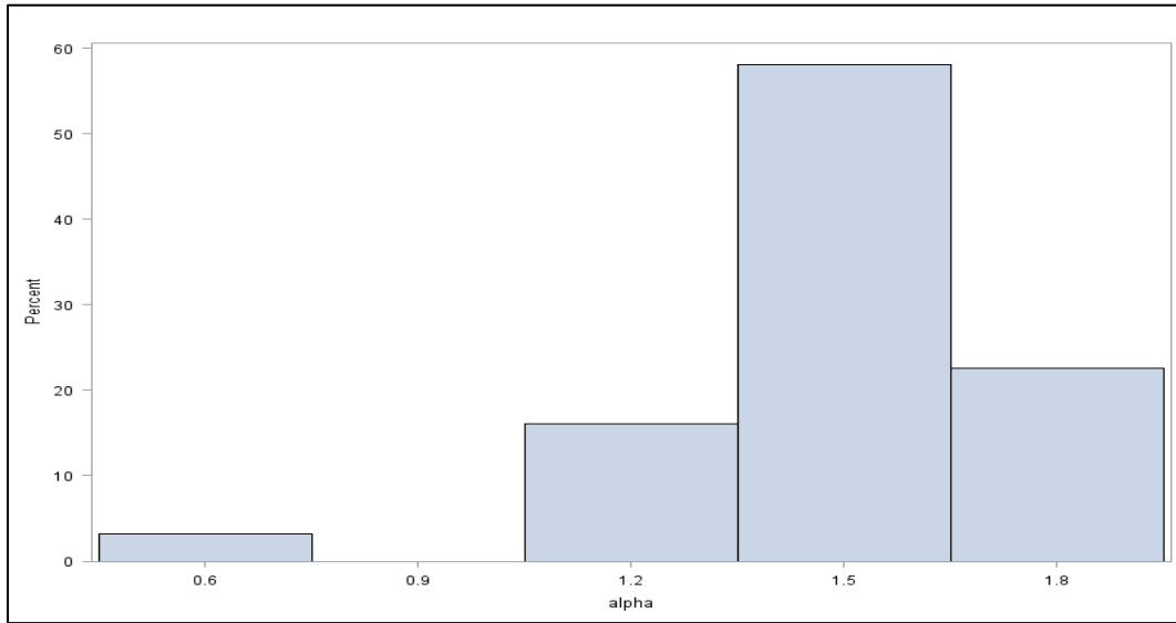
Figure 1. Distribution of the stability index \alpha for log-returns distribution of the selected assets
