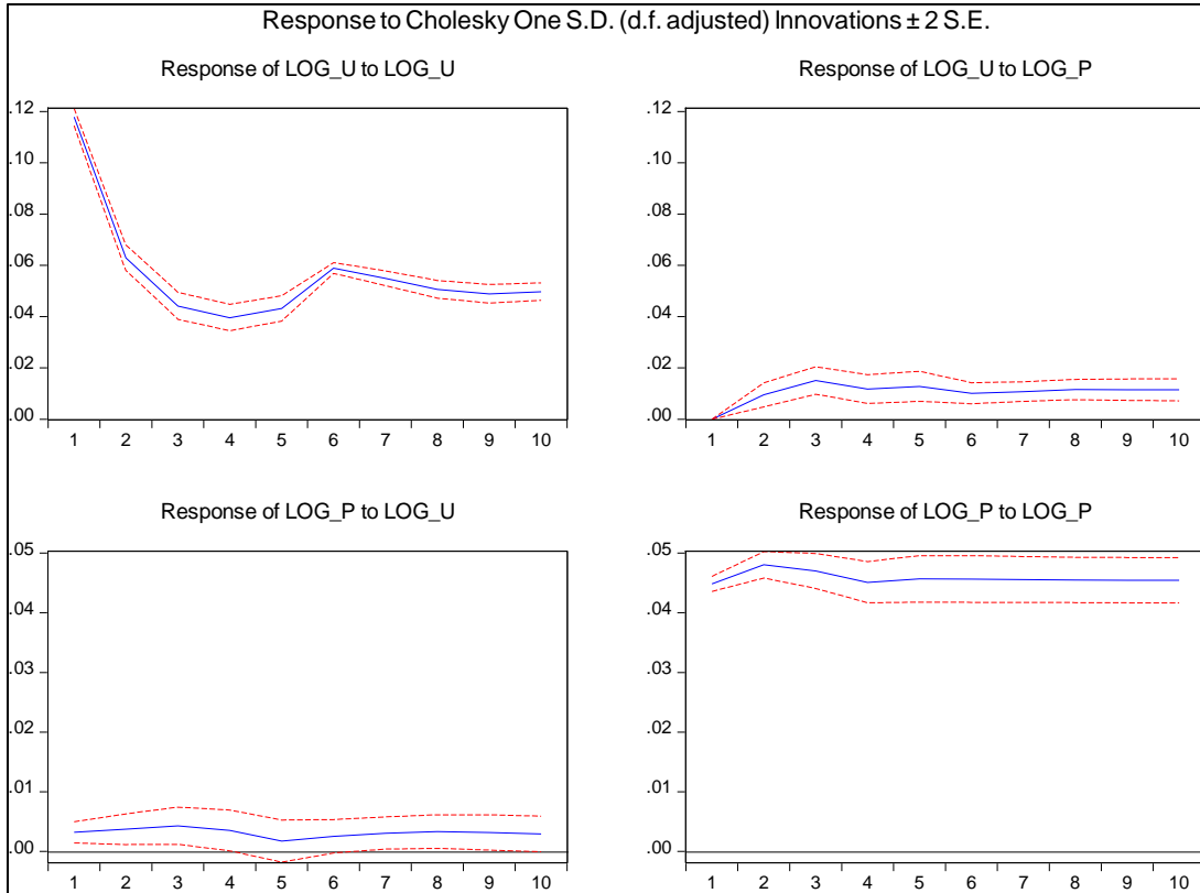
Figure 8. Impulse Response Function for the estimated VAR model
